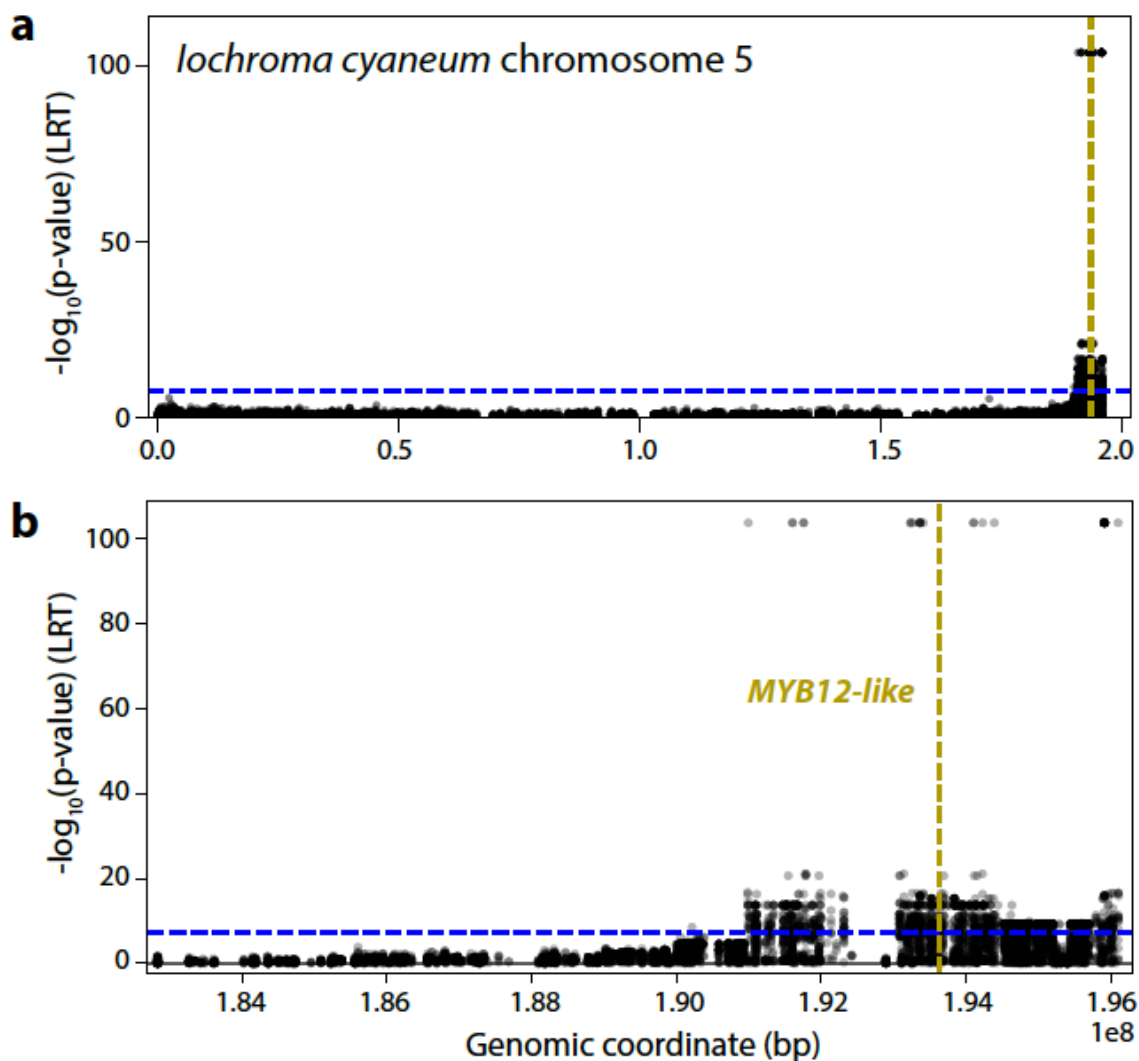
Fig. 2. Manhattan plot showing significant SNP associations on lochroma cyaneum chromosome 5. The blue-dashed line marks the cutoff for genome-wide significance ( P < 5 \times 10^{-8} ). The gold vertical line marks the location of the MYB12-like gene, which predicts F3'H expression. a) The position of MYB12-like near the 3' prime end of the chromosome. b) Close-up of the region containing MYB12-like , showing the concentration of associated SNPs in the last 500kb of the chromosome.
