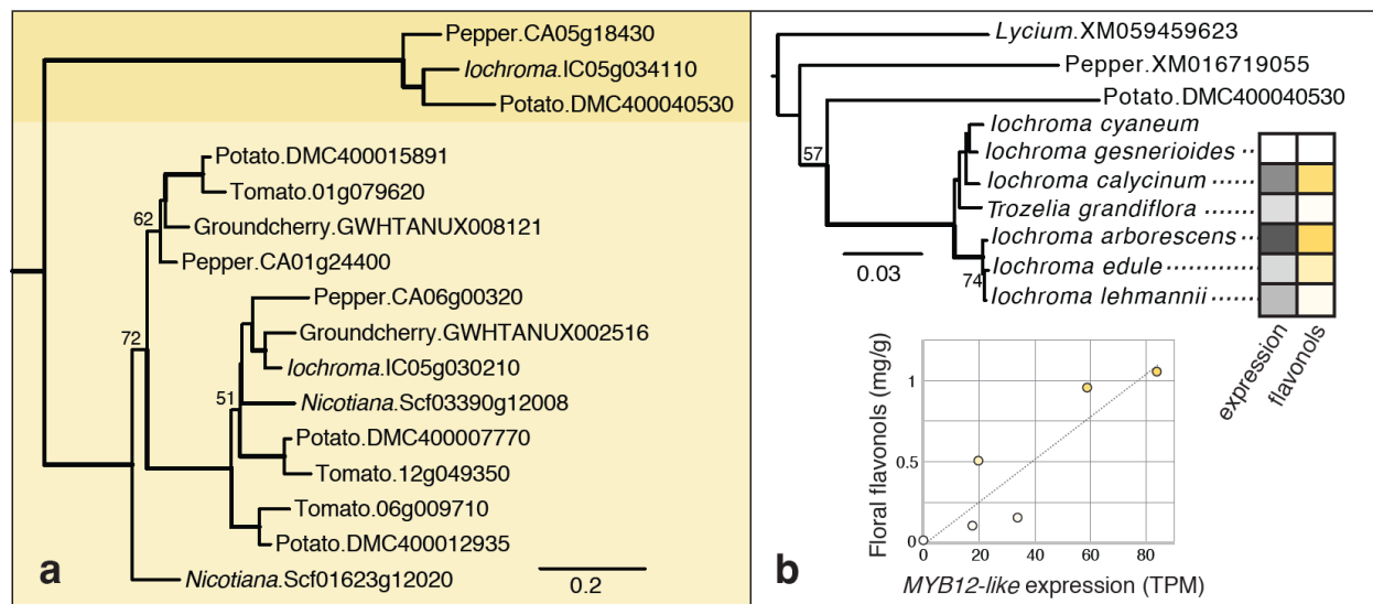
Fig. 4. Phylogenetic relationships among Solanaceae subgroup 7 (SG7) MYBs. a) Maximum likelihood phylogeny from amino acid sequences; the sequences highlighted in light yellow include the best studied SG7 MYBs in Solanaceae, e.g., SMYB12 (Tomato.01g079620) that is tied to the colorless fruit epidermis phenotype (Ballester et al. 2010). The deeply diverged MYB12-like sequences are highlighted in dark yellow; IcMYB12-like corresponds to lochroma .IC05g034110. Bolded branches have >95% bootstrap support; values between 50 and 95% bootstrap support are given. The outgroups used to root the tree (SG7 MYBs from Arabidopsis ) have been pruned. b) Maximum likelihood phylogeny for Solanaceae MYB12-like sequences based on a complete CDS alignment. Bootstrap supports are shown as in (a). Tip values for MYB12-like expression (TPM) and floral flavonol content (in mg/g from Larter et al. 2019) for six species are colored by magnitude (see Supplementary Table 6 for raw data). These data are graphed in the inset figure with the dashed line showing the linear trend. lochroma cyaneum is not included as data from previous transcriptomic analyses (Gates et al. 2018) are not directly comparable with the de novo transcriptomes from the present study. Full names and sources for all sequences used in these analyses are given in Supplementary Table 7. Branch lengths in both trees are in substitutions per site.
