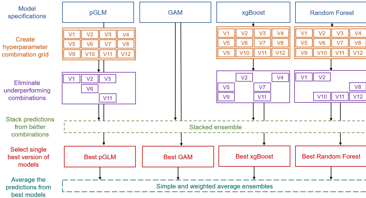
Figure 4: Model flow diagram showing the relationship between base model specifications, hyperparameter combinations and the model ensemble.
