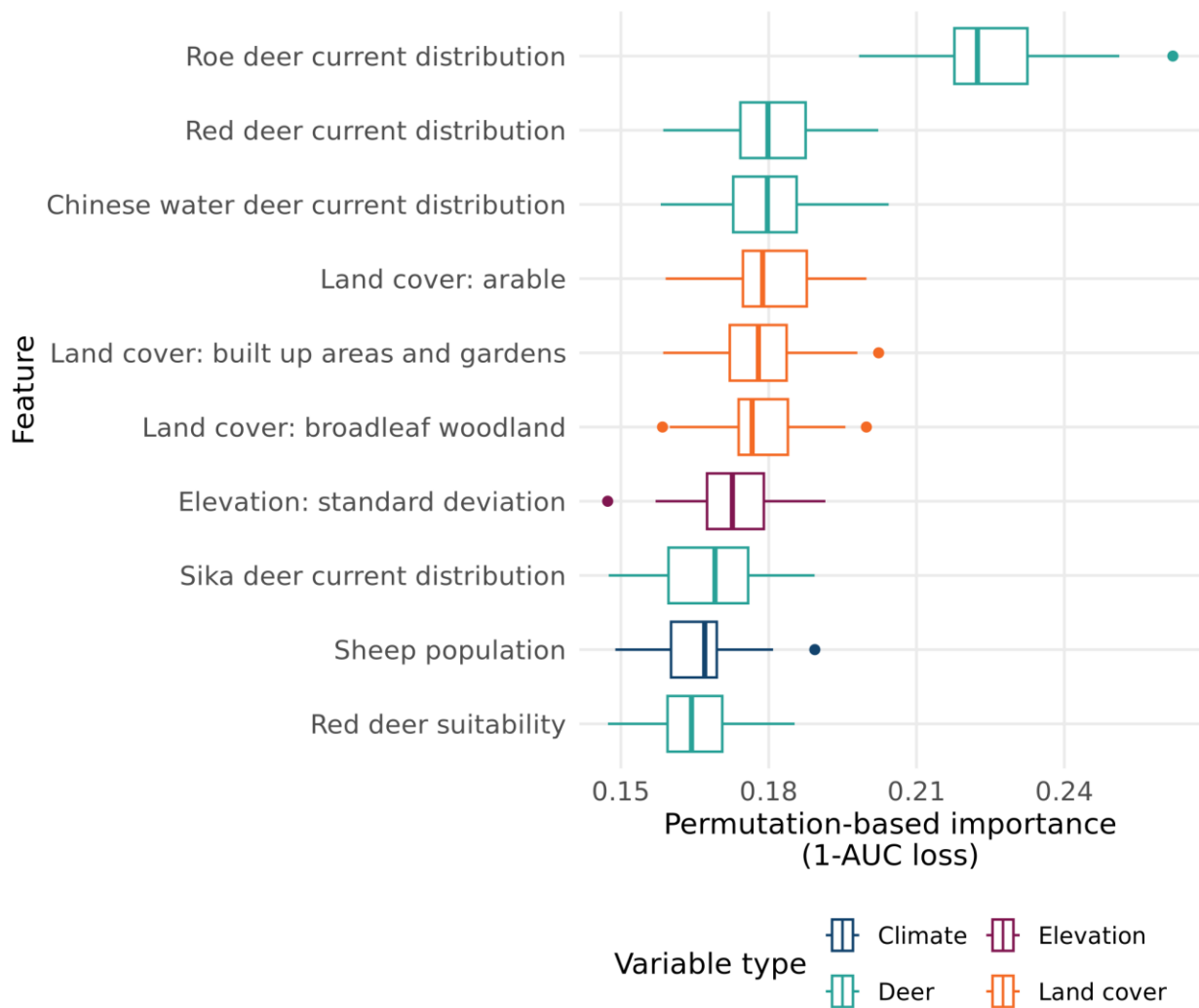
Figure 11: Permutation-based variable importance for simple ensemble predictions on the testing set. The plot shows the ten most important variables on average across 25 iterations, along with confidence intervals. Loss is measured as impact on 1-ROC AUC.
