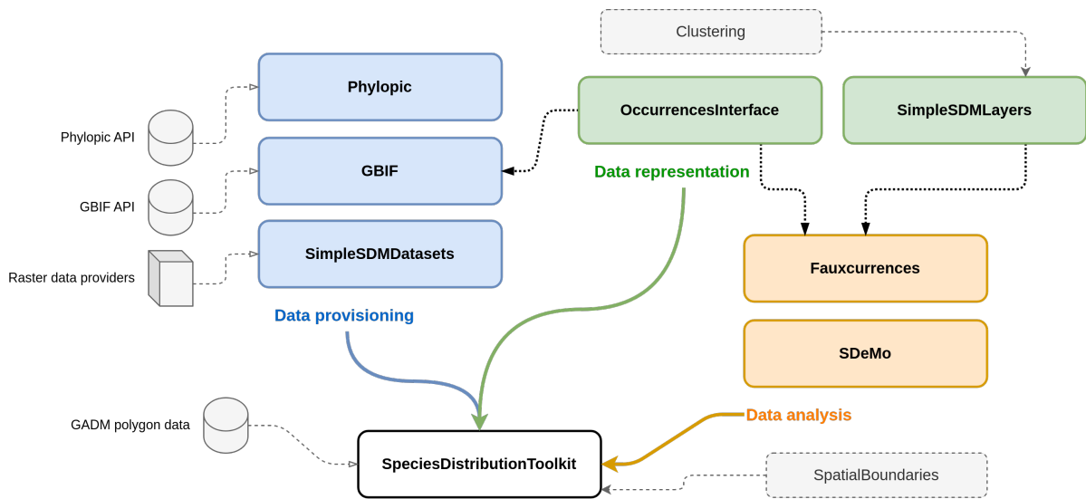
Figure 1: Overview of the packages included in SpeciesDistributionToolkit . The packages are color-coded by intended use (acquisition, representation, and analysis of data). The specific content of each package is presented in the main text. Note that because the package relies on interfaces to facilitate code interoperability, there are only three dependency relationships (black arrows). Some packages can interact with data sources, represented on the left side of the figure. When loading SpeciesDistributionToolkit , all public methods from the package are accessible to the user. Packages that are supported through extensions are in dashed boxes.
