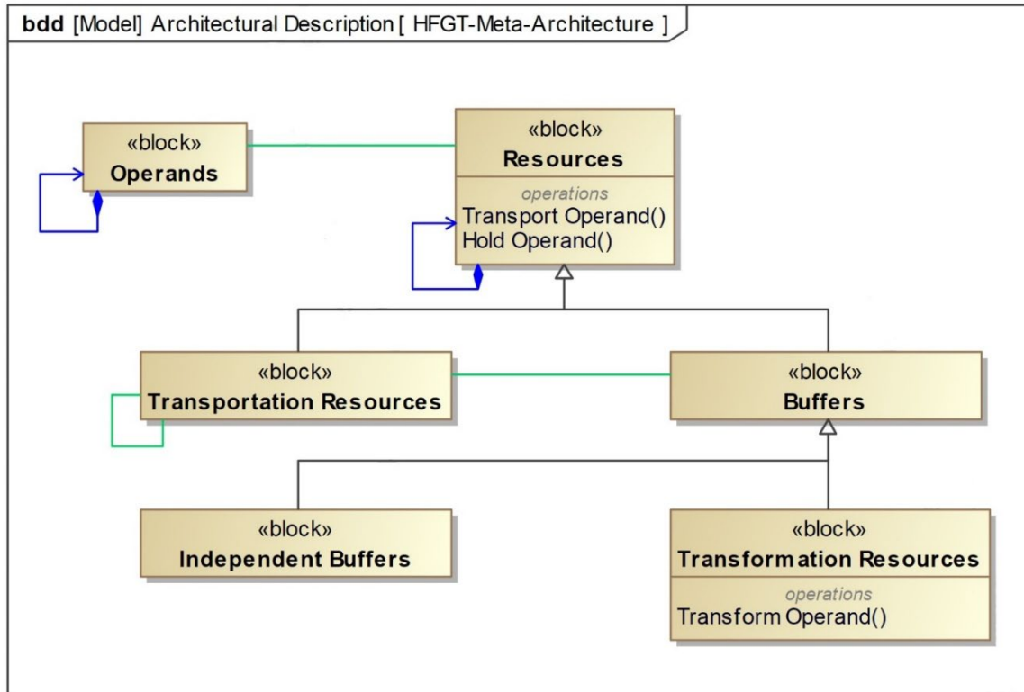
Figure 6. The hetero-functional graph theory (HFGT) meta-architecture [142] represented using the systems modeling language (SysML). The HFGT meta-architecture consists of three types of resources (transportation resources, independent buffers and transformation resources) that are capable of two types of processes (transport operand, which implicitly includes hold operand, and transform operand). Lines between the blocks indicate various associations that define structural relationships and visually represent how system elements are connected or composed [141].
