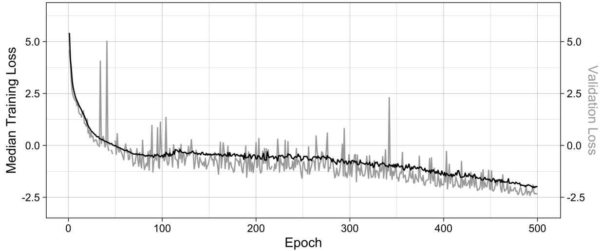
Figure S5. The median training loss of the BayesFlow model (left y-axis, in black) and the validation loss on the testing set (right y-axis, in grey) over the 500 epochs of training. The curves have roughly the same trajectory and plateau towards the end of training, showing that the model has converged and has good generalization to the testing set. Note that the validation loss curve is noisier and lower (on average) than the median training loss curve because it shows only the final value in each epoch, rather than the median value across the entire epoch.
