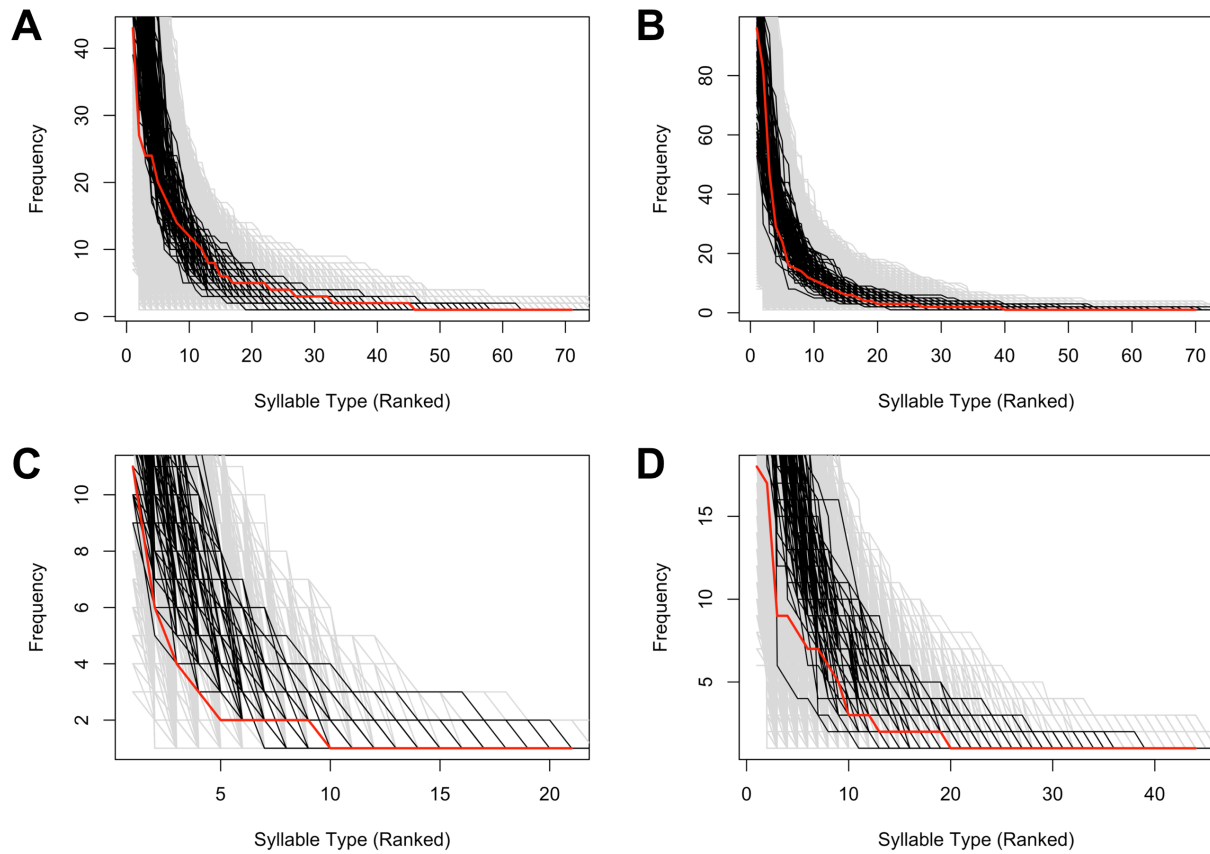
Figure S4. The observed (red) and simulated (grey and black) frequency distributions from 2017 - 2019 for each of the four regiolects (A: Western; B: Eastern; C: Nova Scotia; D: Newfoundland). The black lines denote the 100 simulated distributions with parameter values closest to the estimated parameter values in terms of Euclidean distance. In all cases, the posterior simulations are reasonably close to the observed distribution.
