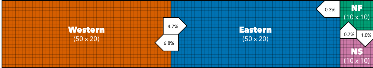
Figure S2. A diagram of the four grids used to simulate geography in the agent-based model, labelled by regiolect. The white arrows denote probability of cultural transmission between neighboring regiolects, based on the proportion of males in each regiolect who sing alien songs averaged across the three time periods (see Supplementary Material Table S3 above for more details).
