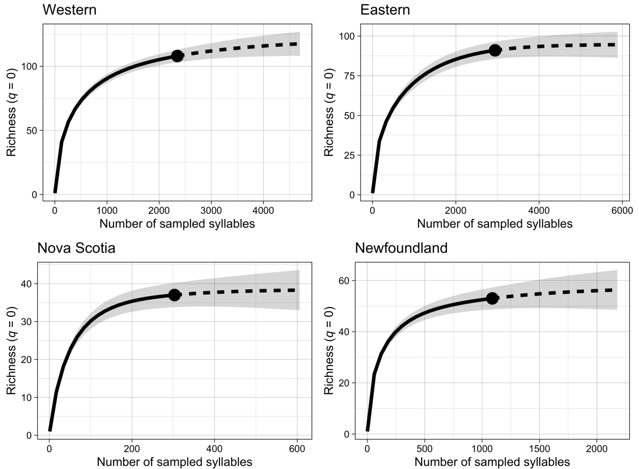
Figure S3. The results of unseen species models applied to the full frequency distribution of syllables in each regiolect across all yrs, run using the iNEXT package in R (Hsieh et al. 2016). The point in each plot marks the observed richness ( y -axis) for the total number syllables sampled ( x -axis). The solid lines mark interpolated richness, the dashed lines mark extrapolated richness, and the shaded areas mark 95% confidence intervals. The interpolated richness values are the number of types you observe if you subsample that number of tokens from the real data. The extrapolated values are the projected number of types you would observe if you were able to continue sampling tokens from the same population. More details can be found in Hsieh et al. 2016: https://doi.org/10.1111/2041-210X.12613 ). We appear to have nearly complete coverage of syllable types in each regiolect.
