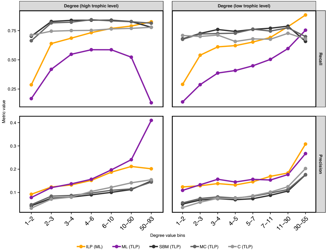
Fig. 3: Comparison of model performance across node degrees. The ILP model provides more effective guidance for discovering missing links compared with non-machine-learning transductive models by consistently maintaining higher precision, ensuring that identified potential interactions are more likely to be validated in the field. While achieving comparable recall at intermediate to high node degrees, the ILP model excels at extremes of node degree—specialist interactions at low degrees and interactions with limited information at high degrees. Compared with the machine-learning-based transductive (TLP) model, the ILP model offered similar precision but substantially higher recall, further enhancing its practical utility for targeted ecological sampling efforts.
