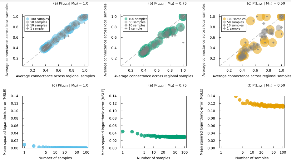
Figure 4 Connectance of sampled binary interaction networks. (a-c) Average connectance of binary interaction networks obtained from the two sampling techniques for 20 randomly selected host-parasite networks. Cross markers represent the connectance of a single sample for each network, diamond markers the average connectance across 10 samples, hexagon markers the average connectance across 50 samples, and the colored circles the average connectance across 100 samples (marker size proportional to the number of samples). (d-f) Reduction in the mean squared logarithmic error between the average connectance of binary interaction networks (all 233 host-parasite networks) obtained from these two sampling techniques as the number of samples increases. The local probability of interaction between potentially interacting species was set to three different values: (a,d) P(L_{i,j,k}|M_{i,j}) = 1.0 , (b,e) P(L_{i,j,k}|M_{i,j}) = 0.75 , and (c,f) P(L_{i,j,k}|M_{i,j}) = 0.50 . Probabilities of regional interactions were obtained with a false positive rate of 5% and a false negative rate of 10%. Regional samples were obtained by randomly sampling binary interactions from the probabilistic interaction metaweb, and then propagating this result to all local networks that include the species potentially engaged in the interactions. Local samples were obtained by independently sampling binary interactions for each local network of probabilistic interactions.
