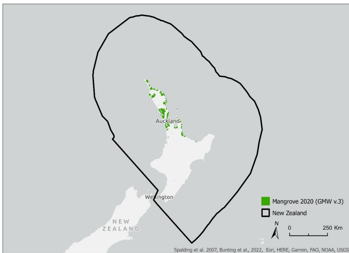
Figure 1. The distribution of mangroves in New Zealand (shown in green). Source: 2020 Mangrove extent extracted from Bunting et al. , 2022. Province limits modified from Spalding et al. , 2007.
