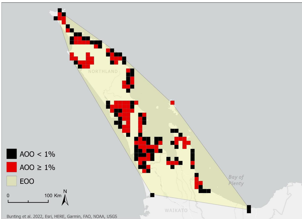
Figure 3. The New Zealand mangrove Extent Of Occurrence (EOO) and Area Of Occupancy (AOO) in 2020. Estimates based on 2020 GMW v3.0 spatial layer (Bunting et al. , 2022). The red 10 x 10 km grids (n=100.) are more than 1% covered by the ecosystem, and the black grids <1% (n= 91).
