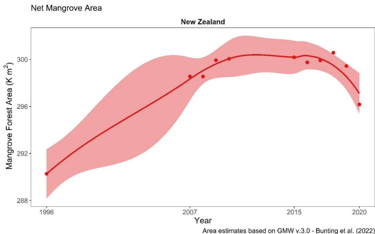
Figure 2. New Zealand mangrove ecosystem between 1996 to 2020. Circles represent the province mangrove area between 1996 and 2020 based on the GMW v3.0 dataset and equations in Bunting et al. , (2022). The solid line and shaded area are the loess smoothing and 95% confidence intervals.
