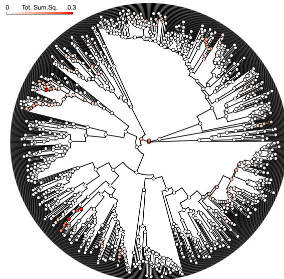
Figure S6: Depicting uncertainties (as total sum of squares) in the ancestral state estimation across six different reconstructions (maximum likelihood, stochastic mapping and hidden
