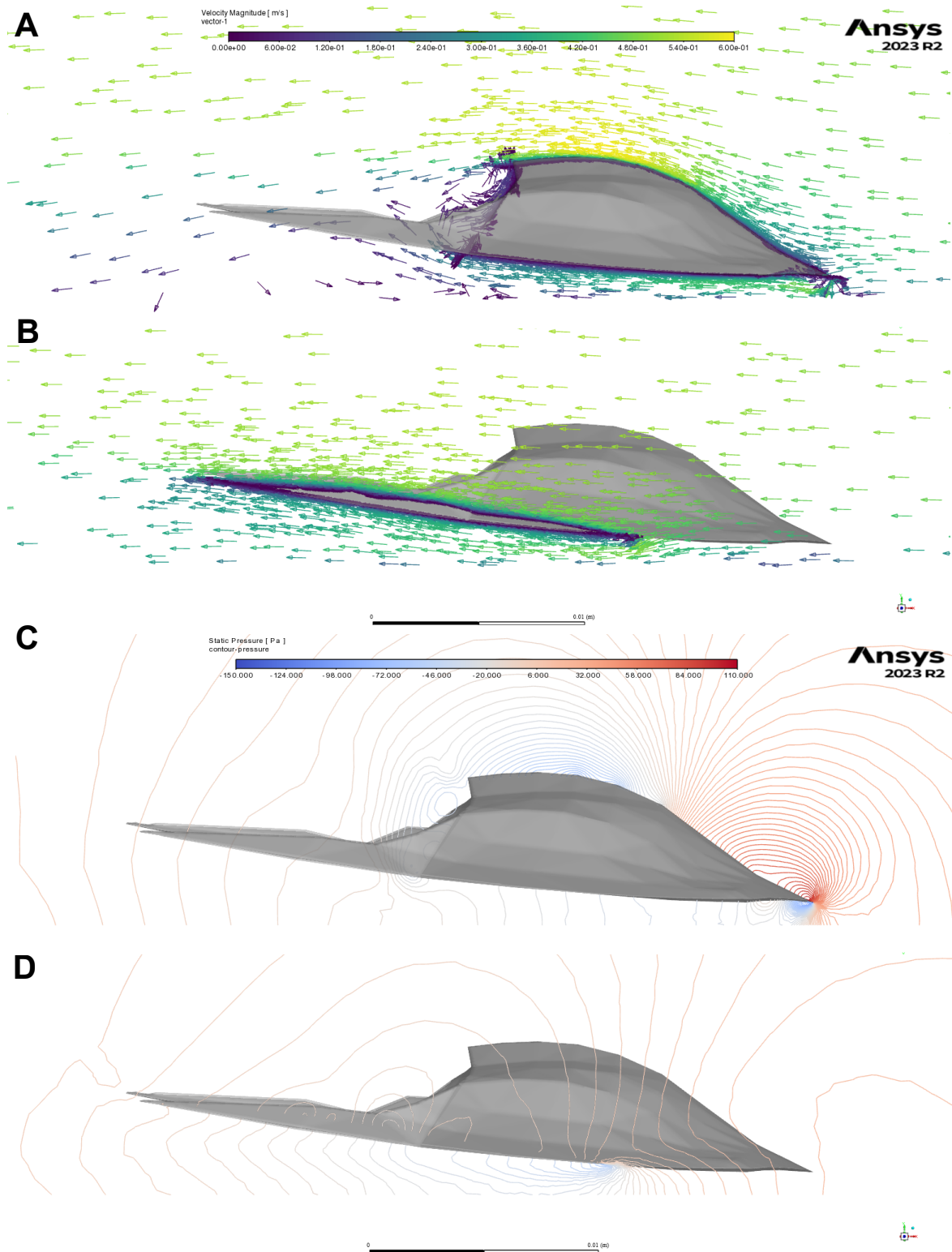
Figure 1: Example CFD simulation to test palaeoecological hypotheses; simulated flow around a hypothetical harped trilobite cephalon, to analyse the hydrodynamic importance of the genal prolongations. A, simulated velocity, projection taken through axial midline of trilobite; B, simulated velocity, projection taken through right-hand genal prolongation; C, simulated pressure, projection taken through axial midline of trilobite; D, simulated pressure, projection taken through right-hand genal prolongation. Images reproduced from Pates & Drage (2024).
