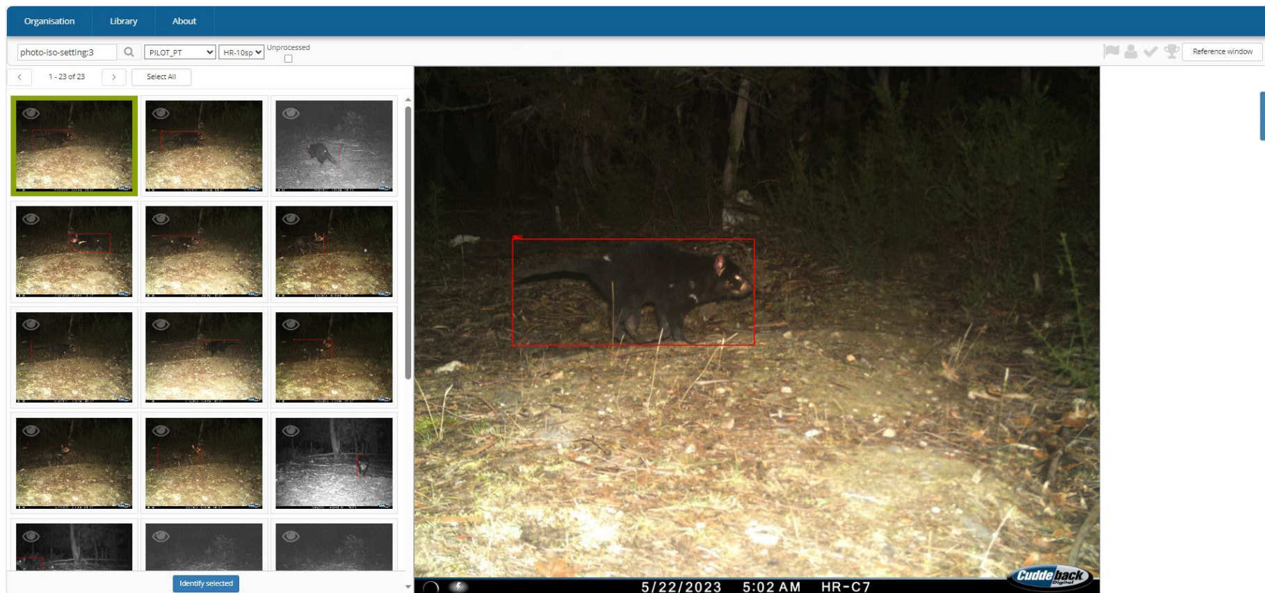
Figure 5. Example screenshot from the Camelot camera-trap database software, showing the use of the MEWC-encoded meta-data to automatically sort the images by species. This allows for efficient viewing and bulk validation by human experts following the preliminary machine classification (if deemed necessary). In this example the species code (#3) for the Tasmanian Devil is written to the ISO field of the metadata and can be searched in Camelot without any modifications to this software. This system also works well in other popular image-tagging software such as ExifPro 18 or Timelapse 19 .
