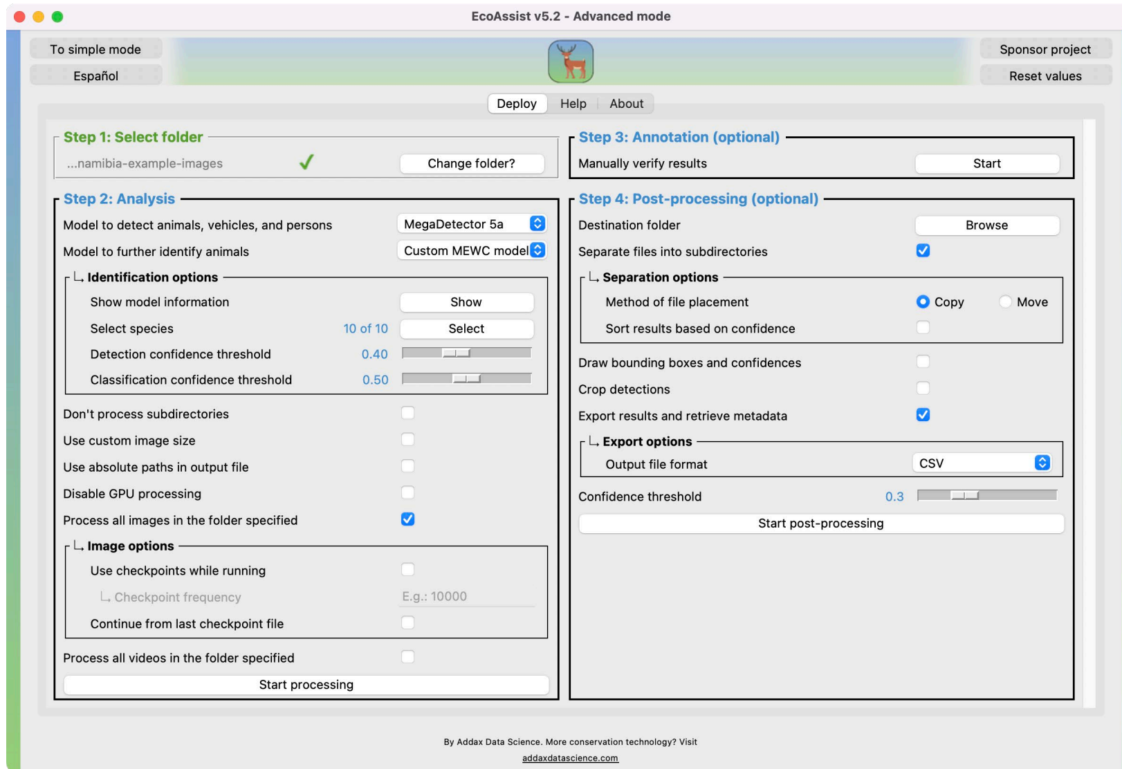
Figure 6. Example screenshot from the EcoAssist application, showing the features for deploying MEWC models.
