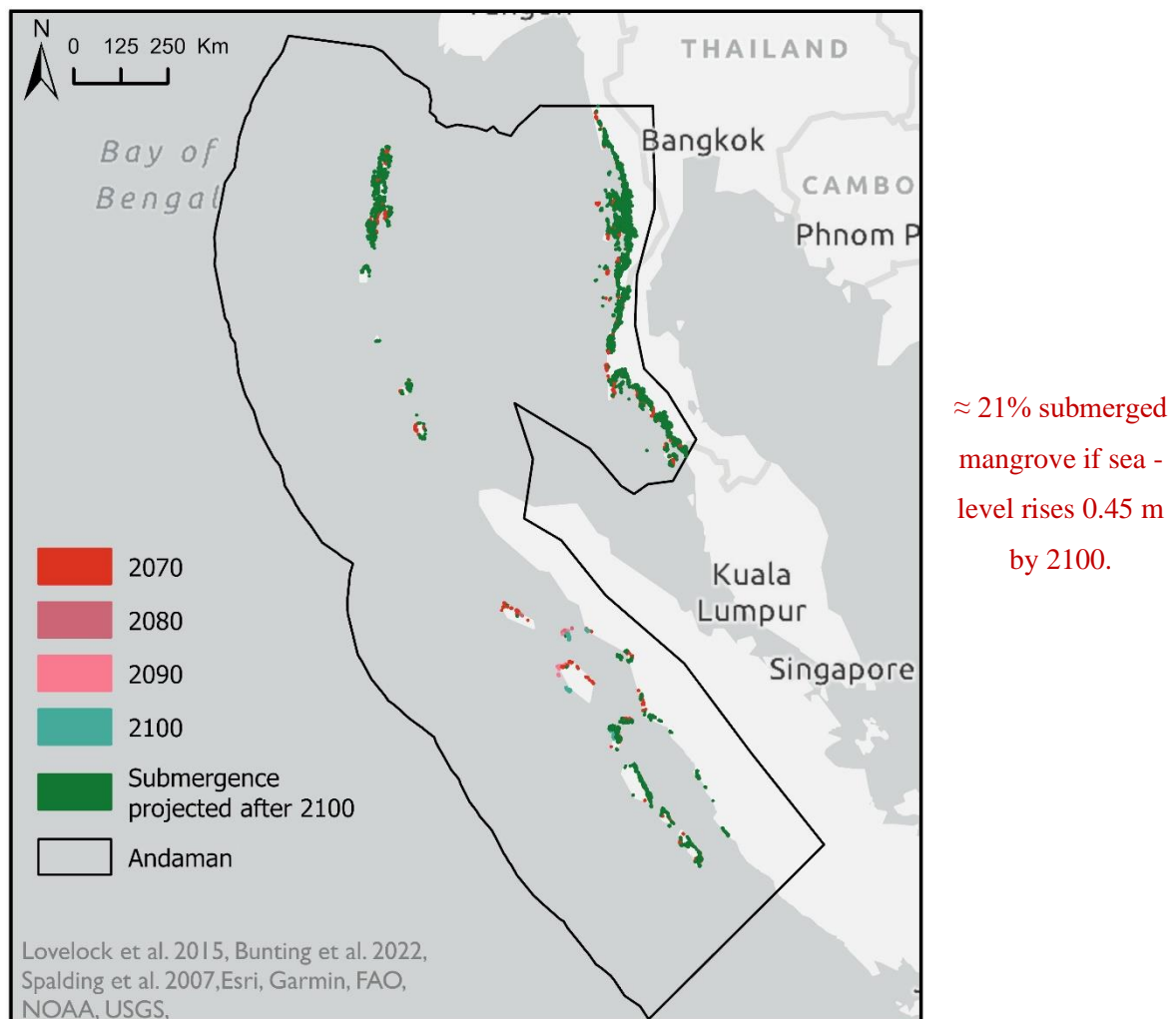
Figure 3. Andaman mangrove forest predicted decade of submerge under IPCC RCP 6 scenario (0.45 m Global SLR by 2100), based on the model of Lovelock et al. (2015). Mangrove extent based on 2020 GMW v3.0 spatial layer (Bunting et al. , 2022).
