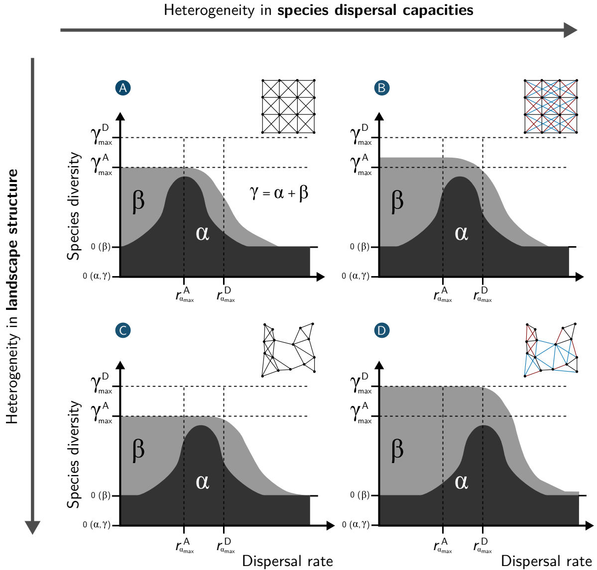
Figure 2: Dispersal heterogeneity underlies biodiversity variation. Respective levels of \alpha (dark grey area), \beta (light grey area), and \gamma diversities (sum of \alpha and \beta , represented by the total dark and light grey area); and their hypothetical responses to increases in dispersal rates in homogeneous (A) and heterogeneous (B, C, D) dispersal networks. When dispersal rates increase, communities usually shift from being affected by dispersal limitation to maximising \alpha diversity when species can optimally track resources. In the former case, communities eventually become homogenised when dispersal is not limited, and strong competitors tend to dominate. In a homogeneous dispersal network (A), \alpha diversity is maximised at a dispersal rate r_{\alpha_{max}}^A , and the maximum \gamma diversity is \gamma_{max}^A .
