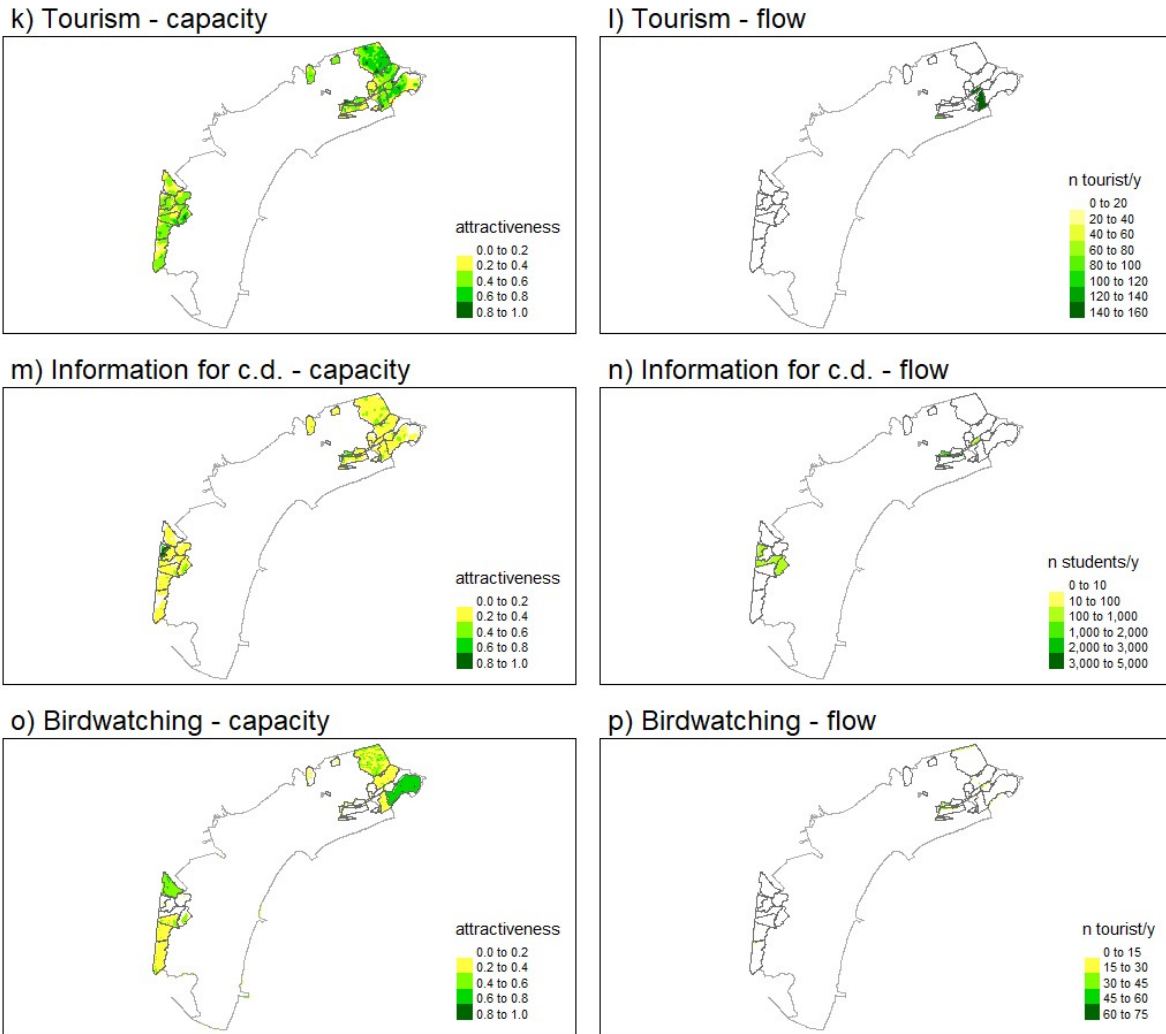
Fig. S.M. IV Results of the ESs assessment. a), b), c), d) refer to regulating and maintenance ESs. e), f), g), h), i), j) refer to provisioning ESs. k), l), m), n), o), p) refer to cultural ESs.
