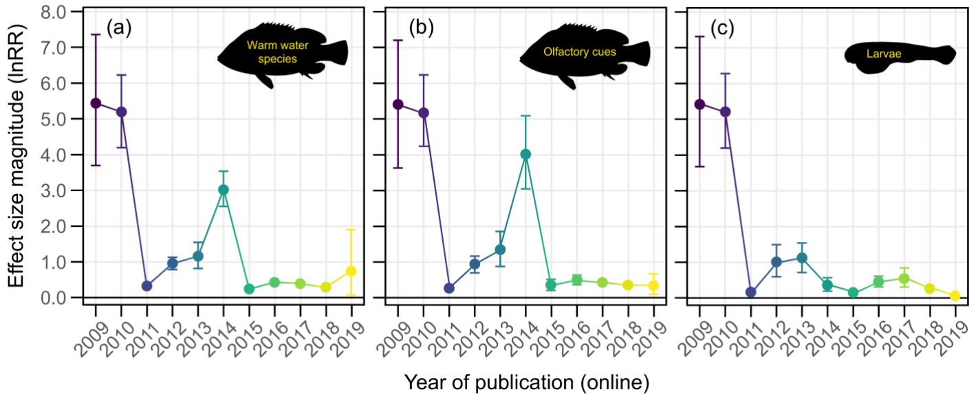
Fig 2. The decline effect cannot be explained by three commonly-considered biological drivers of acidification effects. Mean effect size magnitude (absolute lnRR \pm upper and lower confidence bounds) as a function of time for datasets that only included experiments with (a) warm-water species, (b) olfactory-associated behaviours, and (c) larval life stages. Mean effect size magnitudes and confidence bounds were estimated using Bayesian simulations and a folded normal distribution. Note: colours are aesthetic in nature and follow a gradient according to year of publication. Source data for each figure panel can be found in Supplementary File 14.
