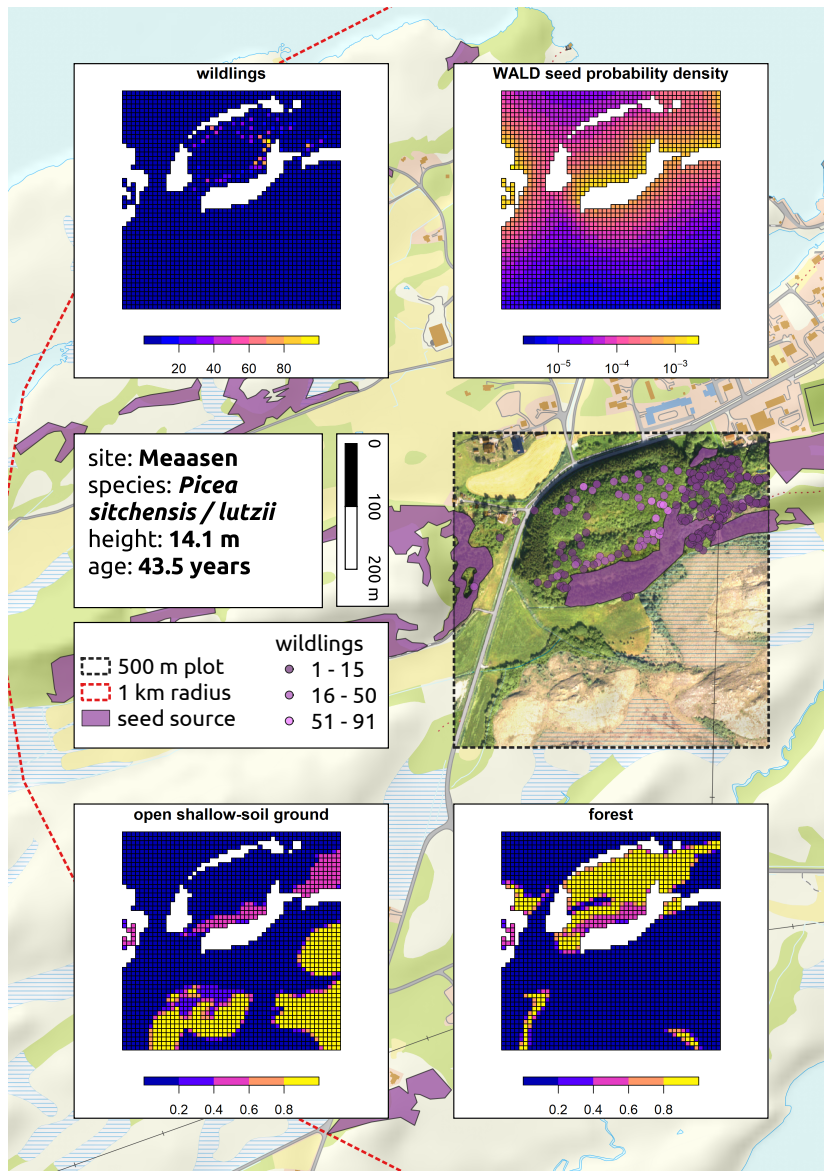
Figure 2: An illustration of one of the 82 plantations: Meaasen. The background map shows the surroundings of the plantation, and the 500x500 m plot is overlaid with an aerial photograph. The middle row of panels shows data as registered in the field. The top and bottom rows of panels show selected variables for the 500x500 m plot, as used in the regression model (with a spatial grain of 10 m). Grid cells without data are either seed sources or "tree plantations" of other species.
