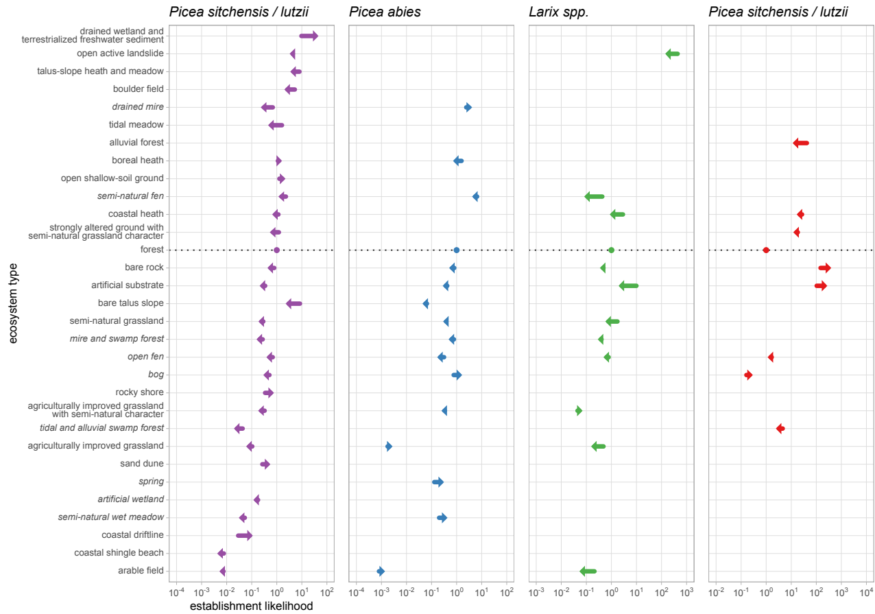
Figure 6: Shifts in estimated relative establishment likelihoods when relative seed rain (from the WALD dispersal model) is included in the model as a covariate rather than an offset. Arrows point from the models with offsets to the models with covariates.
