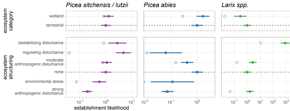
Figure 5: Relative densities (unfilled points) and relative establishment likelihoods (filled points) of three alien conifer species groups among categories of ecosystem types (top) or structuring processes in ecosystem types (bottom). Relative establishment likelihoods are shown with 95 % confidence intervals. The horizontal dotted lines indicate the reference strata.
