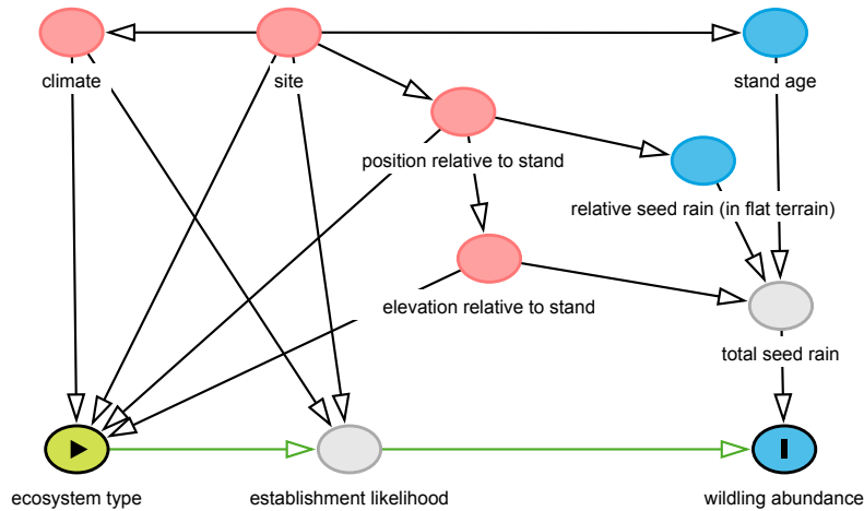
Figure 3: A directed acyclic graph showing the assumed causal relationships motivating our statistical model of ecosystems’ effects on wildling abundance. Red variables causally affect both the ecosystem type and wildling abundance, blue variables causally affect only wildling abundance, and grey variables are unobserved. Green arrows show the causal pathway of interest.
