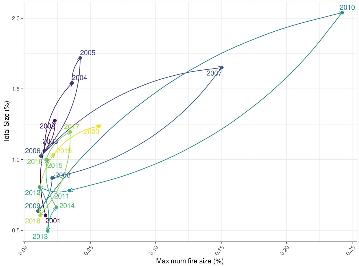
Figure 1: Annual total fire size vs maximum fire size for the Amazon as a percent of the region area. Estimated with MODIS burned area product. These observed data exhibit cycles of loading and discharge, years with high fire extension and big fire events—the upper right region of the figure—which are followed by years of low fire extension and no extreme events in the lower left region. A typical trajectory could be the years 2009, 2010 and 2011 where this cycle can be clearly observed.
