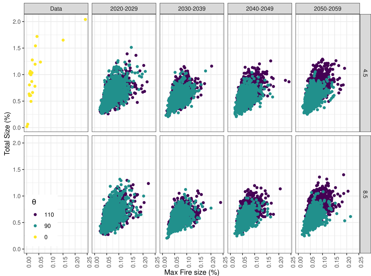
Figure 4: Total annual size of fires vs maximum fire size % relative to the area of the region. The data column was estimated using MODIS burned area product. The predictions by decade were estimated with a fitted model using a monthly ignition probability calculated with data from General Circulation Models under two greenhouse gas emissions scenarios known as Representative Concentration Pathways (RCPs), RCP4.5 and RCP8.5. From the best fitted fire models we show two with the minimum and maximum \theta parameter.
