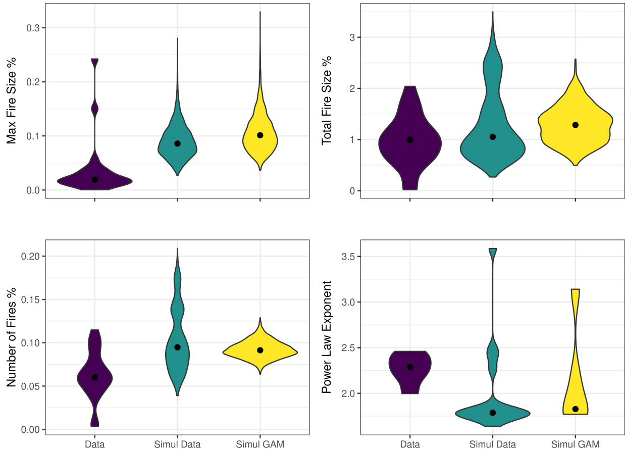
Figure 3: Predictions of the fire model compared with data for the years 2001-2020. We used best-fit parameters, the ignition probability from MODIS, and the ignition probability from the estimated GAM models (Simul GAM), to run the model. All the outputs are relative to the total area; black points are the medians.
