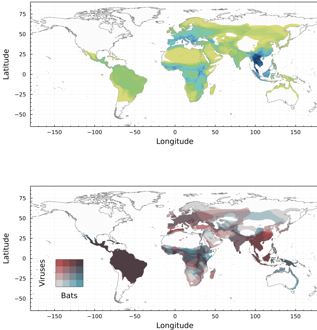
Figure 2 Bat and betacoronavirus diversity. Top panel: relative diversity of known bat hosts of betacoronaviruses. This map shows that the region with the largest number of possible hosts is South-Eastern Asia. Bottom panel: congruence between the evolutionary distinctiveness of the hosts (grey to blue) and the viruses (grey to red).
