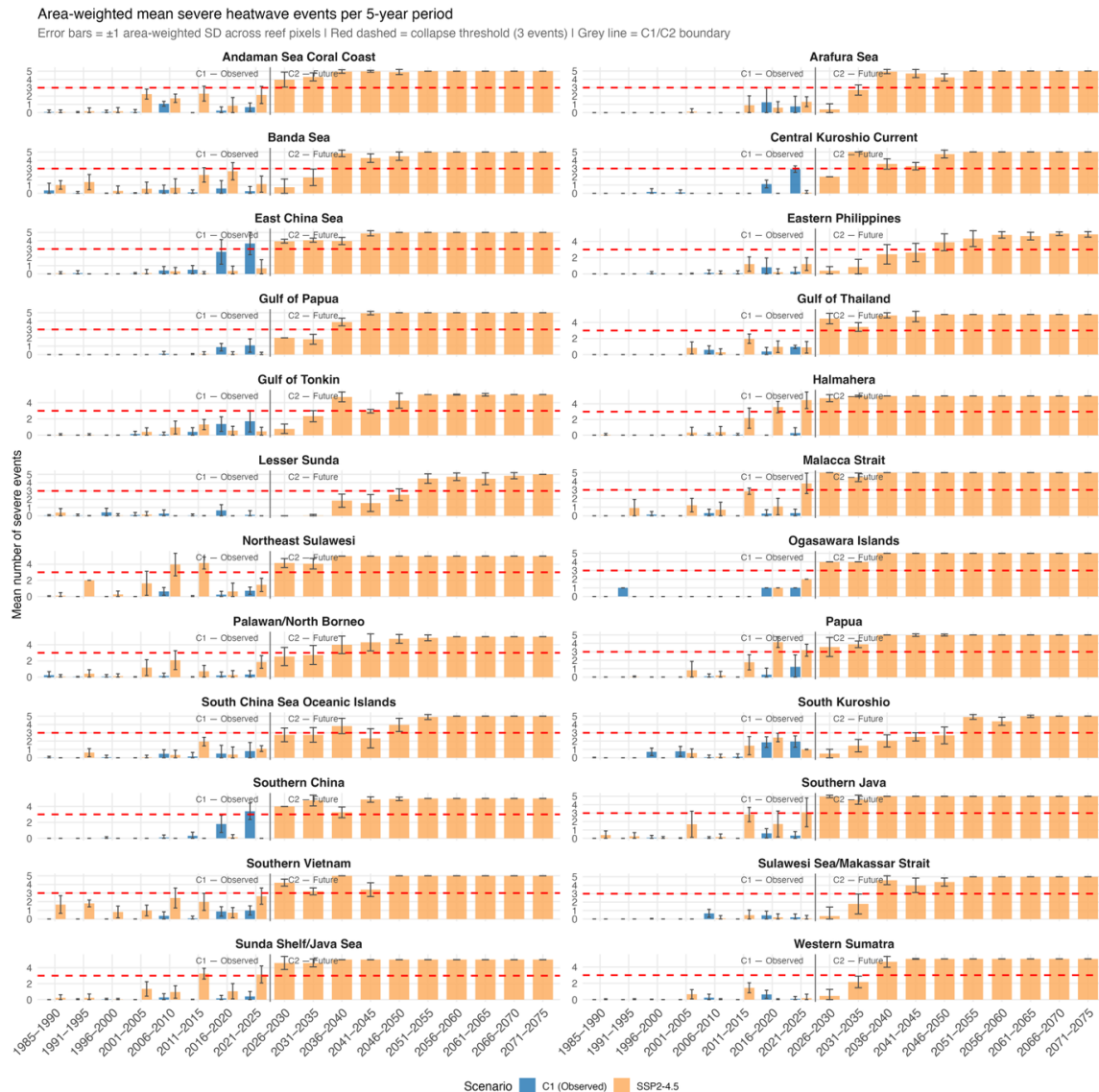
Figure S18. Mean number of severe mortality events per 5-year period, averaged across coral reef pixels within each ecoregion, under two trajectories: observed data used to assess sub-criterion C1 (blue bars, 1985–2025) and projections under SSP2-4.5 (orange bars, 1985–2075). Severe mortality events are defined as years in which annual maximum DHW exceeded ecoregion-specific acute stress thresholds associated with widespread coral mortality. Error bars represent \pm 1 SD across reef pixels within each ecoregion, reflecting spatial variability in the frequency of severe thermal exposure. The red dashed horizontal line indicates the collapse threshold of 3 severe mortality events within a 5-year window. The vertical grey line marks the boundary between the observed (C1, 1985–2025) and projected (C2, 2026–2075) assessment periods.
