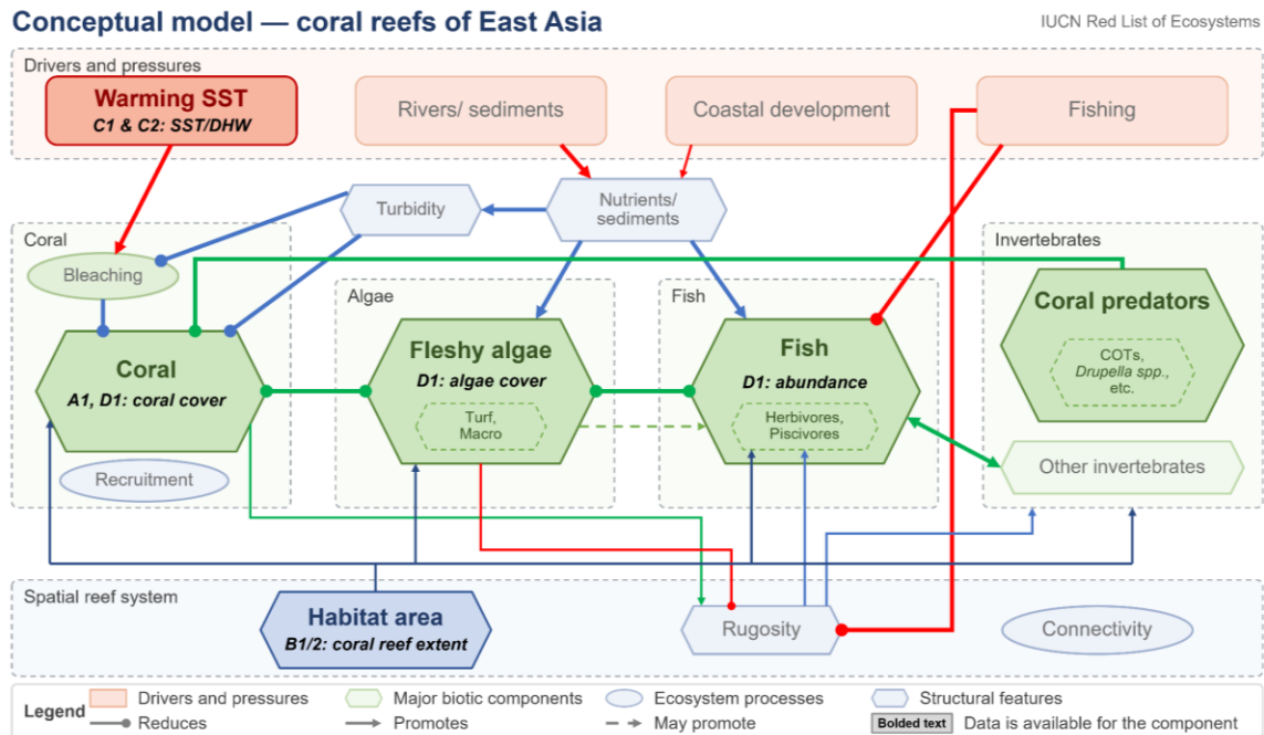
Figure 4 | Conceptual model of East Asia's coral reef ecosystems. The model illustrates key biotic and abiotic components, as well as external drivers, threats, and the processes and interactions between them. All sub-criteria that have been analyzed are highlighted in italics.
