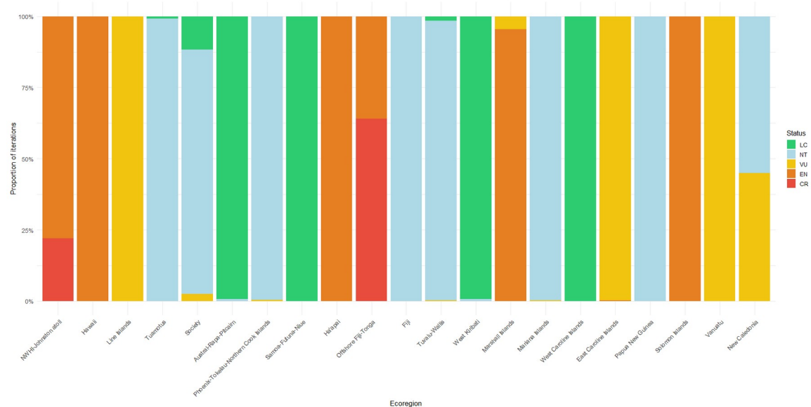
Figure S5. Proportion of 1000 Monte Carlo iterations landing in each IUCN Red List of Ecosystems risk category, by Pacific ecoregion, for Criterion D (hard coral cover) under a 5% collapse threshold.
