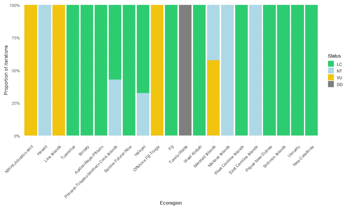
Figure S6. Proportion of 1000 Monte Carlo iterations landing in each IUCN Red List of Ecosystems risk category, by Pacific ecoregion, for Criterion D (macroalgae:coral ratio) under a 0.833 collapse threshold.
