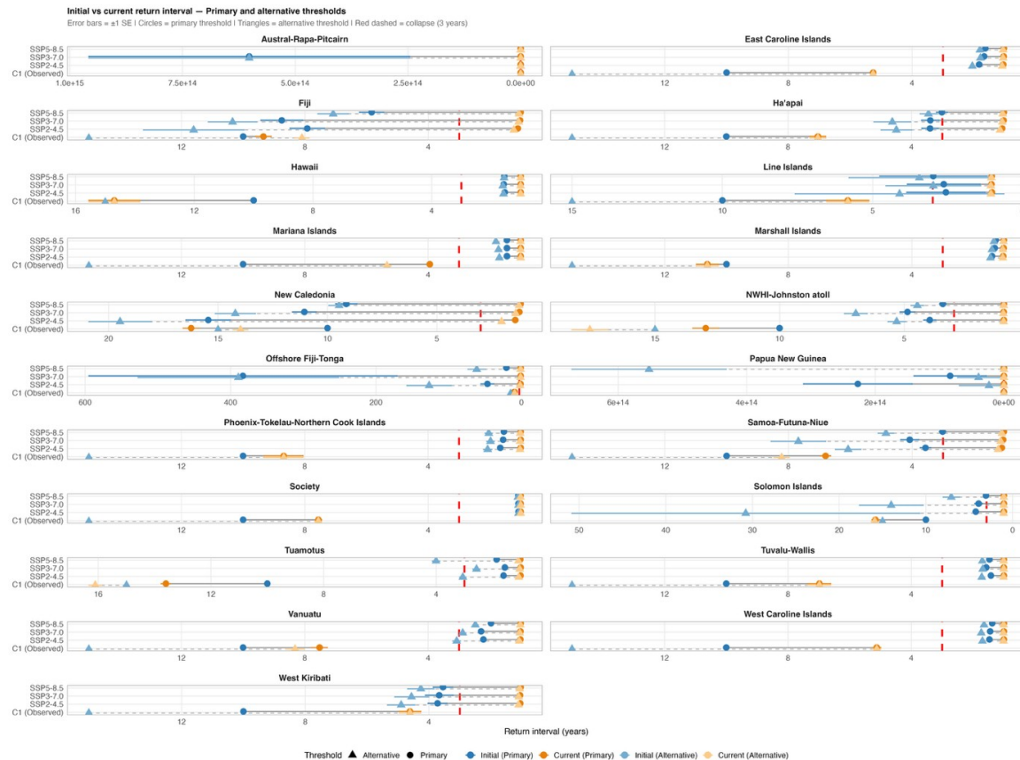
Figure S9. Change in the average return interval between severe bleaching events (years) for each ecoregion (x-axis), comparing initial conditions (blue) to current or projected future conditions (orange) across four trajectories (y-axis): observed data (C1) and projections under SSP2-4.5, SSP3-7.0, and SSP5-8.5. Connecting lines indicate the direction and magnitude of change between initial and current conditions. Return intervals were estimated for the chronic pathway by fitting a binomial regression model to the binary bleaching event time series for each reef pixel, with values representing the shortest return interval identified over each assessment period (C1: 1985–2025; C2: 2026–2075). Results are shown for both primary (filled circles) and alternative (filled triangles) DHW thresholds. For C1, initial conditions are assumed to reflect historical disturbance regimes prior to the satellite record, corresponding to a return interval of 10 years (primary threshold) and 15 years (alternative threshold). For C2, initial conditions are calculated from projected DHW data over 1996–2025 using the same probabilistic model. Error bars represent \pm 1 SE across reef pixels within each ecoregion. The red dashed vertical line marks the collapse threshold of a 3-year return interval, below which disturbance frequency is considered sufficient to prevent meaningful coral recovery and drive progressive ecosystem degradation. Note that the x-axis is reversed such that movement from left to right represents a shortening return interval and worsening conditions.
