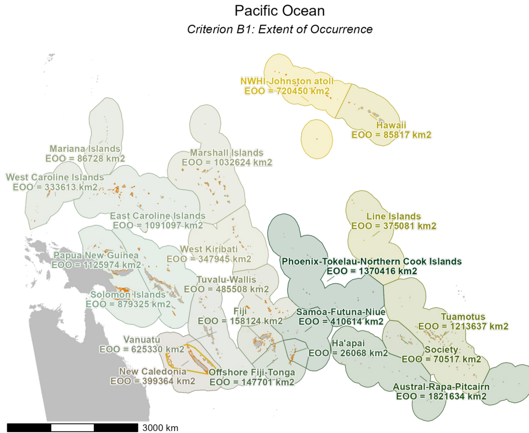
Figure S2. Extent of Occurrence (EOO) by ecoregion under Criterion B1, for the 21 Pacific coral reef ecoregions. EOO is calculated as the minimum convex polygon encompassing all known coral reef occurrences within each ecoregion (km 2 ).
