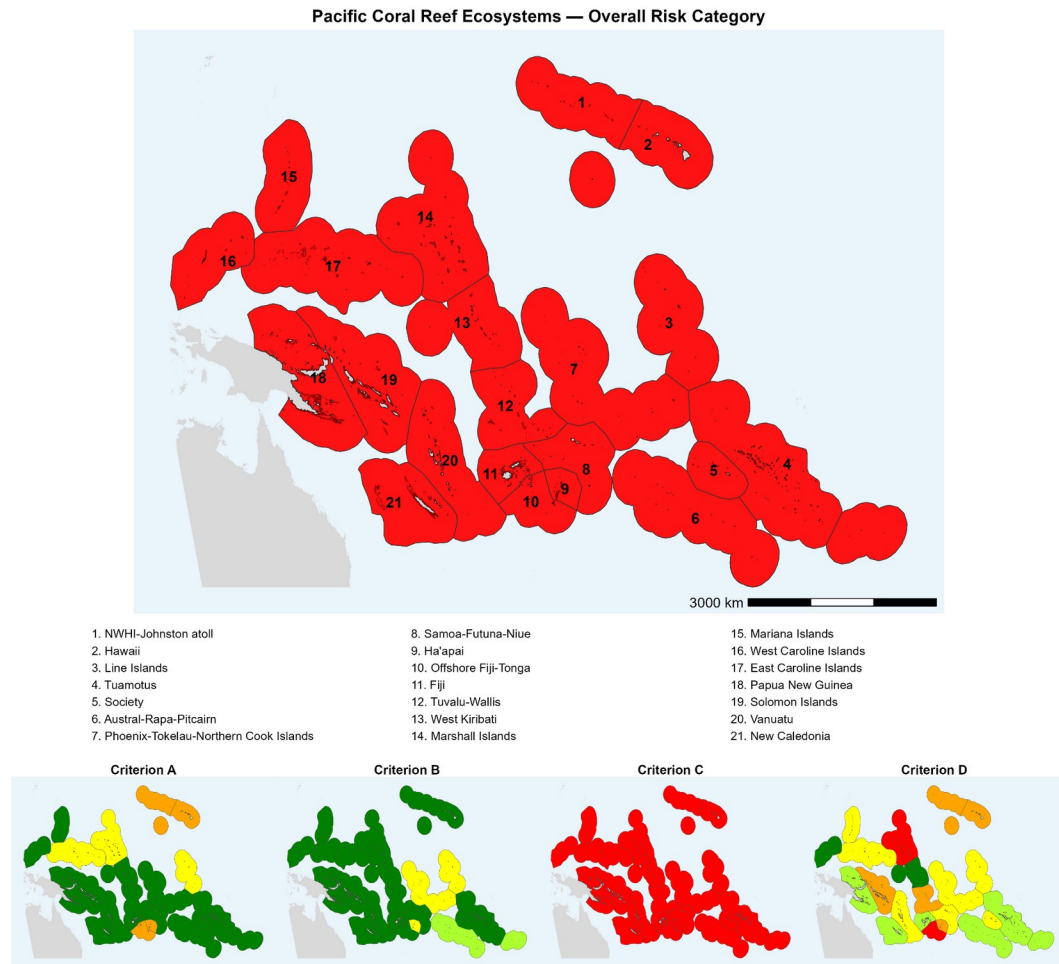
Figure 1. Distribution of the 21 coral reef ecoregions in the Pacific. Map above: overall IUCN Red List of Ecosystems risk status. Maps below : risk status results for Criteria A–D. Risk categories are listed as follows : NE = Not Evaluated, DD = Data Deficient, CO = Collapsed, CR = Critically Endangered, EN = Endangered, VU = Vulnerable, NT = Near Threatened, LC = Least Concern.
