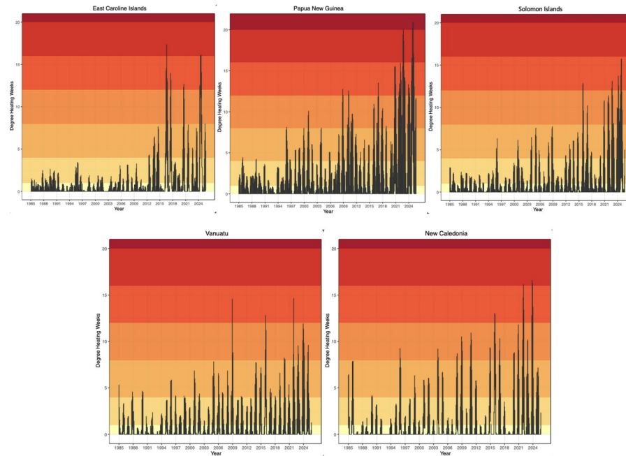
Figure S4. DHW plot by year and ecoregion. Each vertical spike spans the range of DHW values recorded per year for the ecoregion, from observed satellite data.
