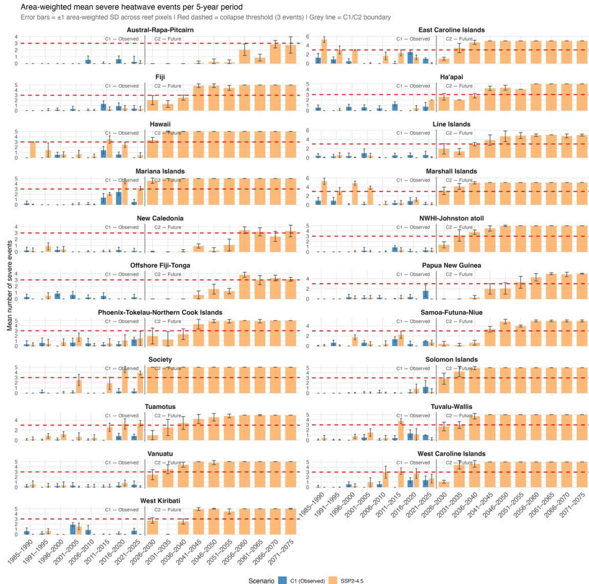
Figure S10. Mean number of severe mortality events per 5-year period, averaged across coral reef pixels within each ecoregion, under two trajectories: observed data used to assess sub-criterion C1 (blue bars, 1985–2025) and projections under SSP2-4.5 (orange bars, 1985–2075). Severe mortality events are defined as years in which annual maximum DHW exceeded ecoregion-specific acute stress thresholds associated with widespread coral mortality. Error bars represent \pm 1 SD across reef pixels within each ecoregion, reflecting spatial variability in the frequency of severe thermal exposure. The red dashed horizontal line indicates the collapse threshold of 3 severe mortality events within a 5-year window. The vertical grey line marks the boundary between the observed (C1, 1985–2025) and projected (C2, 2026–2075) assessment periods.
