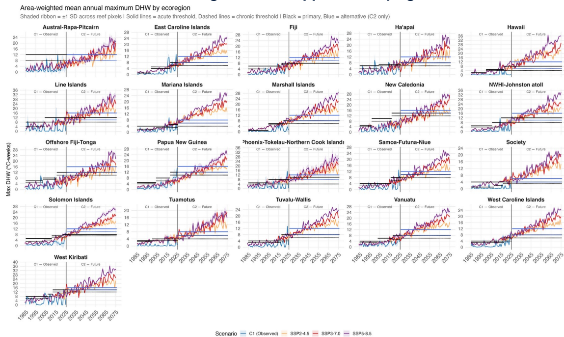
Figure S8. Annual maximum Degree Heating Weeks (DHW) averaged across coral reefs within each ecoregion from 1985-2075 for four trajectories: observed data used to assess sub-criterion C1 from 1985-2025 (blue line), and projections under three Shared Socioeconomic Pathways — SSP2-4.5 (orange), SSP3-7.0 (red), and SSP5-8.5 (purple). Shaded ribbons represent \pm 1 SD in DHW across reef pixels within each ecoregion, reflecting spatial variability in thermal exposure. Horizontal lines show ecoregion-specific DHW thresholds at various points in time corresponding to severe bleaching events (chronic stress pathway; dashed lines) and severe mortality events (acute stress pathway; solid lines). Black lines indicate primary thresholds, and blue lines indicate alternative thresholds (C2 period only, 2026–2075). The vertical grey line marks the boundary between the observed (C1 - 1985-2025) and projected (C2 - 2026-2075) assessment periods.
