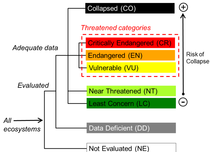
Figure 6. IUCN Red List of Ecosystems categories and assessment pathway. All ecosystem types are evaluated against the assessment criteria and assigned to one of eight categories. Ecosystems with adequate data are classified as Collapsed (CO), Critically Endangered (CR), Endangered (EN), Vulnerable (VU), Near Threatened (NT), or Least Concern (LC), according to their estimated risk of ecosystem collapse.
