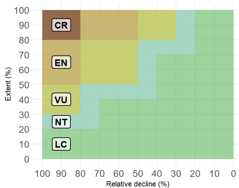
Figure 5. Classification matrix used to evaluate environmental degradation under Criterion C and disruption of biotic processes and interactions under Criterion D of the IUCN Red List of Ecosystems.
