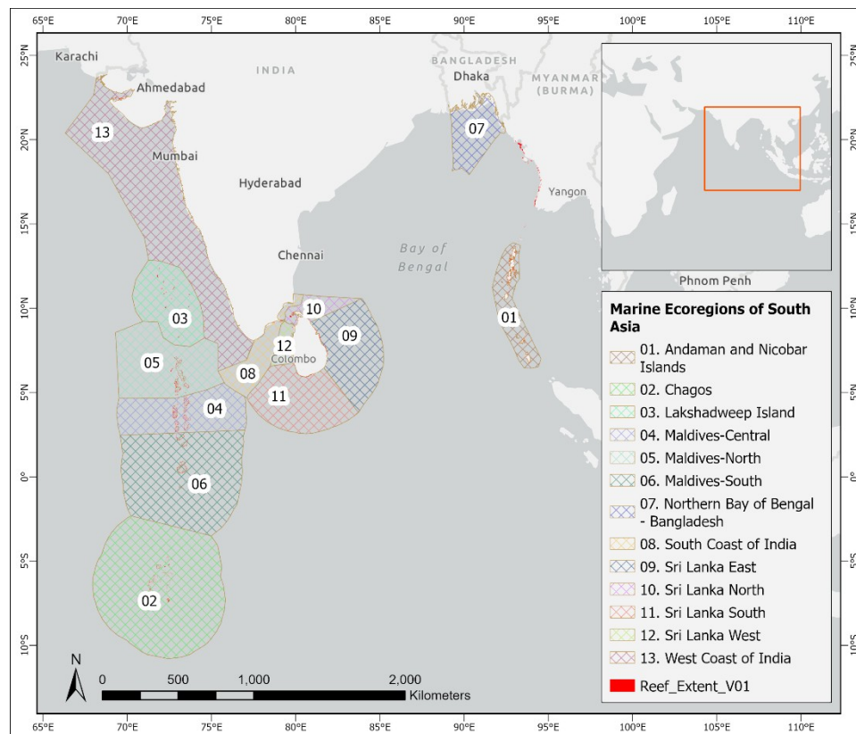
Figure 2. Coral reefs of South Asia, grouped within 13 coral reef ecoregions to be evaluated under the IUCN Red List of Ecosystems criteria and corresponding to Level 4 of the IUCN Global Ecosystem Typology.
