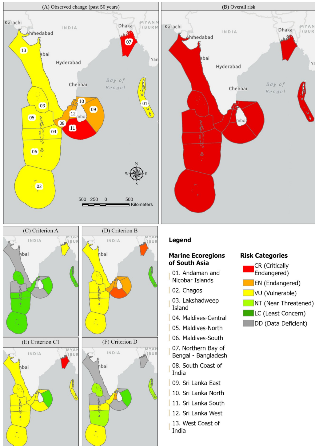
Figure 1. Distribution of the 13 coral reef ecoregions in South Asia. Panel A: Observed change, risk of collapse based on the past 50 years of observed change (criteria A, B, C1 and D). Panel B: Overall Red List of Ecosystems risk status, including projected heat stress over the next 50 years (criterion C2, IPCC SSP2-4.5). Panels C–F: risk status under criterion A (reduction in geographic distribution), criterion B (restricted geographic distribution), criterion C1 (environmental degradation, observed) and criterion D (disruption of biotic processes and interactions).
