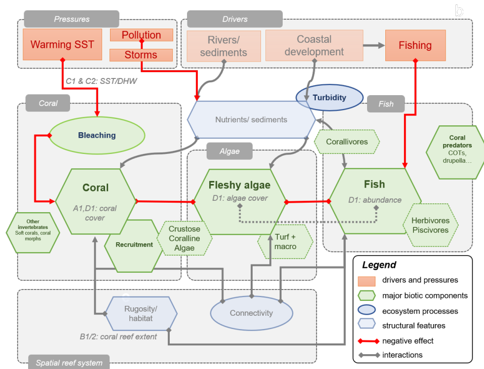
Figure 3. Conceptual model of the South Asia coral reef ecosystems. The model illustrates key biotic and abiotic components, as well as external drivers, threats, and the processes and interactions between them.
