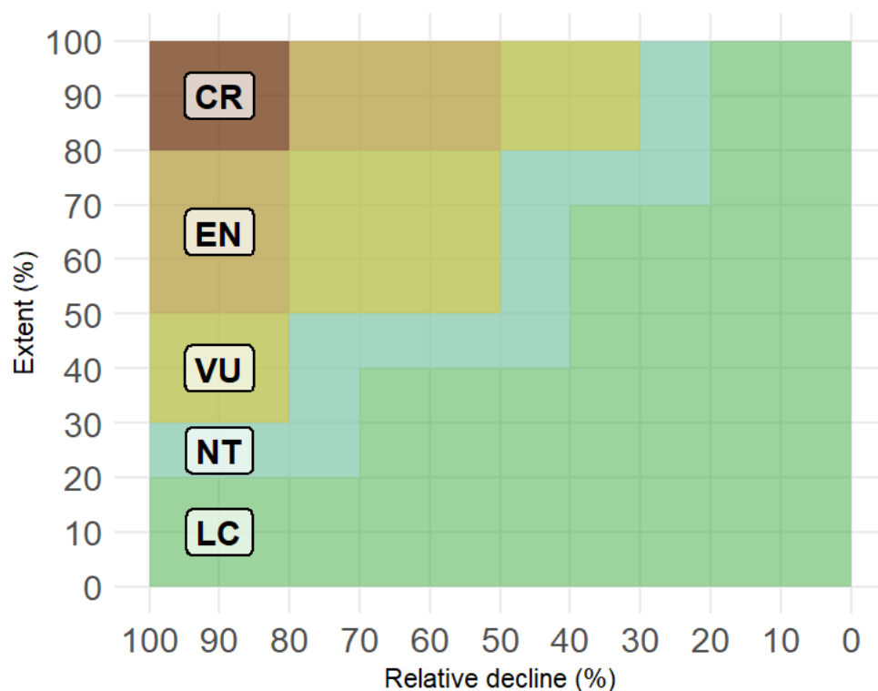
Figure 6. Risk matrix - Relative extent of an ecosystem (y-axis) vs relative severity of decline (x-axis) used to assign risk classifications under Criterion C and D
