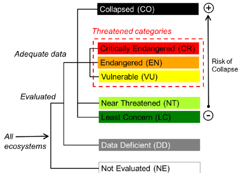
Figure 7. Risk categories for ecosystems from the IUCN Red List of Ecosystems (RLE)
