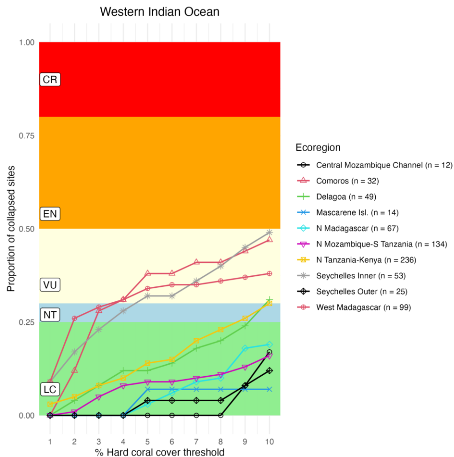
Figure S1. Sensitivity analysis of Criterion A to the collapse threshold for hard coral cover varying from 1% to 10%.
