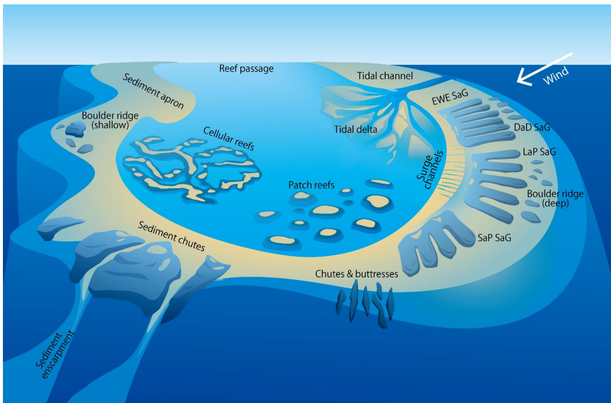
Fig. 3. Schematic representation of cited reef geomorphologies including spur and groove (SaG), following Duce et al. (2016) morphometric classification i) deep and disconnected (DaD), ii) exposed to wave energy (EWE), iii) long and protected (LaP), and iii) short and protected (SaP).
