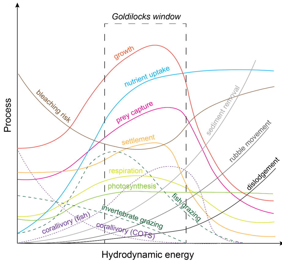
Fig. 9. Representation of the Goldilocks window of reef physiological, ecological and geomorphic processes in relation to hydrodynamic energy. Direction and shape of relationships are hypothesized from the present synthesis.
