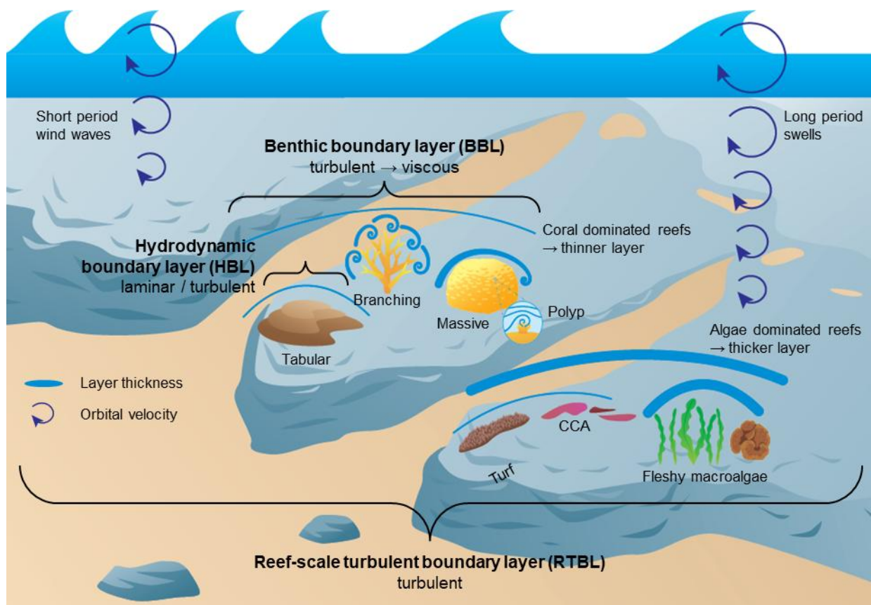
Fig. 1. Conceptual schematic of the hierarchical organization of hydrodynamic boundary layers on coral reefs. The figure illustrates boundary layer structure across nested spatial scales, from the reef-scale turbulent boundary layer (RTBL) to benthic-scale hydrodynamic boundary layers generated by biological roughness. Diffusive and concentration boundary layers are not shown. At the reef scale, boundary-layer thickness
