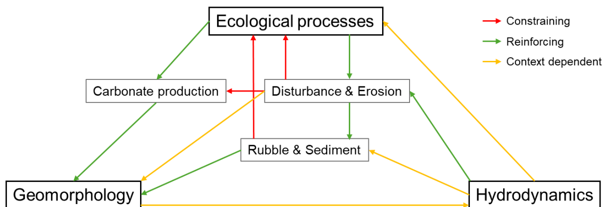
Fig. 8. Ecological processes regulate carbonate production and disturbance, generating loose material that may be used to build reef framework. Geomorphology and hydrodynamics are reciprocally coupled, shaping spatial patterns of flow energy and substrate stability. Feedbacks are classified as constraining (red), reinforcing (green), or context-dependent (yellow), reflecting that many interactions vary in direction and magnitude depending on environmental conditions.
