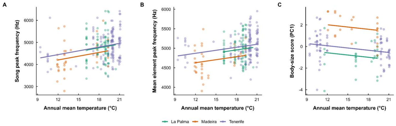
Figure S3. Relationships between annual mean temperature and acoustic and multivariate body-size traits across the three focal islands. (A) Song peak frequency, (B) mean element peak frequency, and (C) multivariate body-size score (PC1) in relation to annual mean temperature (BIO1) in La Palma, Madeira, and Tenerife. In the acoustic panels (A,B), points denote individual birds ( n = 254 : La Palma = 77, Madeira = 38, Tenerife = 139). In the body-size panel (C), points denote individuals with complete data for all four morphological traits included in the PCA ( n = 125 : La Palma = 29, Madeira = 22, Tenerife = 74). Colors indicate island populations. Lines show model-predicted relationships between annual mean temperature and each response variable for each island, restricted to the observed temperature range sampled on that island.
