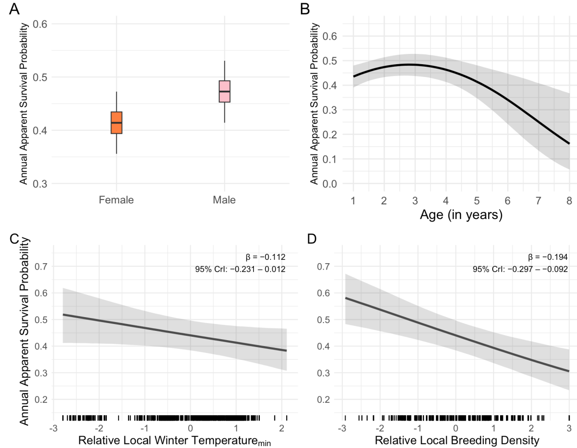
Figure 3: Adult annual apparent survival probabilities according to A) Sex, B) Age, C) Relative local winter minimum temperatures and D) Relative local breeding density. The posterior median and 95% credible intervals are displayed (Table 1). For each fixed effect, the slopes are predicted setting other continuous fixed effects at their mean values and sex at 0.5 to produce a sex-averaged estimate.
