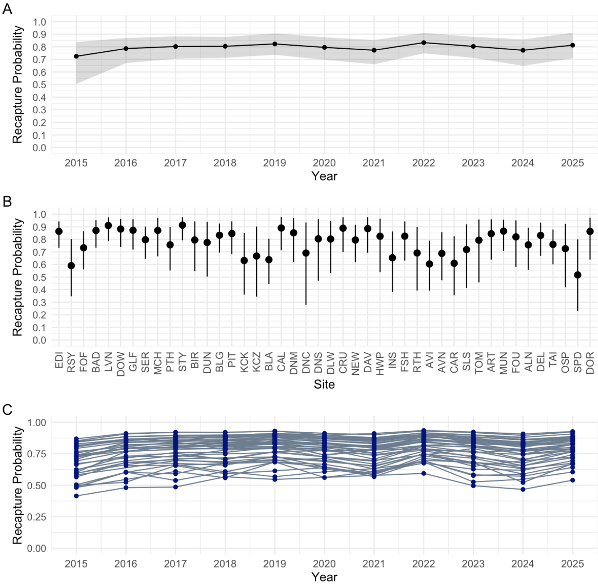
Figure S1: (A) Temporal, (B) spatial and (C) spatiotemporal variation in recapture probability. Posterior median (for A,B, C) and 95% credible intervals (for A, B) displayed (Table 1).
