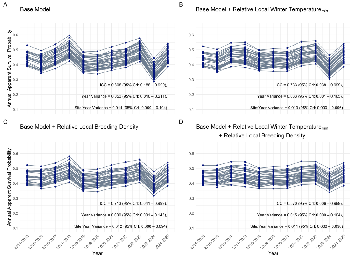
Figure 4: Spatiotemporal patterns in apparent survival probability of adult blue tits obtained from random effect estimates. Coloured lines show the temporal trajectories of mean survival across each of the 44 sites over the 12-year study period. Results presented are from a) base model with fixed effects of sex and age and random effects of site, year and site:year fitted; b) base model plus relative winter minimum temperature; c) base model plus relative local breeding density; d) base model plus relative winter minimum temperature and relative local breeding density. The predictions based on the global intercept plus random effect deviations plus 0.5 \times \text{sex} (producing a sex-averaged estimate, as males and females were coded 0 and 1 respectively) are displayed and they exhibit shrinkage towards the grand mean.
