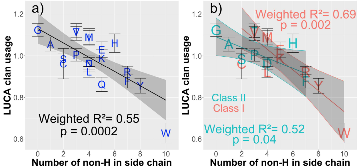
Figure 1. Smaller amino acids were added earlier to the genetic code. LUCA clan usage is from Table 1. In b), glutamine (Q) and asparagine (N) are omitted because the tRNA is charged with glutamate and aspartate, respectively, from which Q or N are produced while bound to tRNA. LysRS-I is presumed to precede LysRS-II, and CysRS to precede SepRS. The squared inverse of the LUCA usage SE values (shown as error bars from Table 1) were used for the ‘weights’ argument in the lm() function within the “stats” package in R, to produce the R^2 and p-values for weighted model 1 regression lines, with 95% CI shading.
