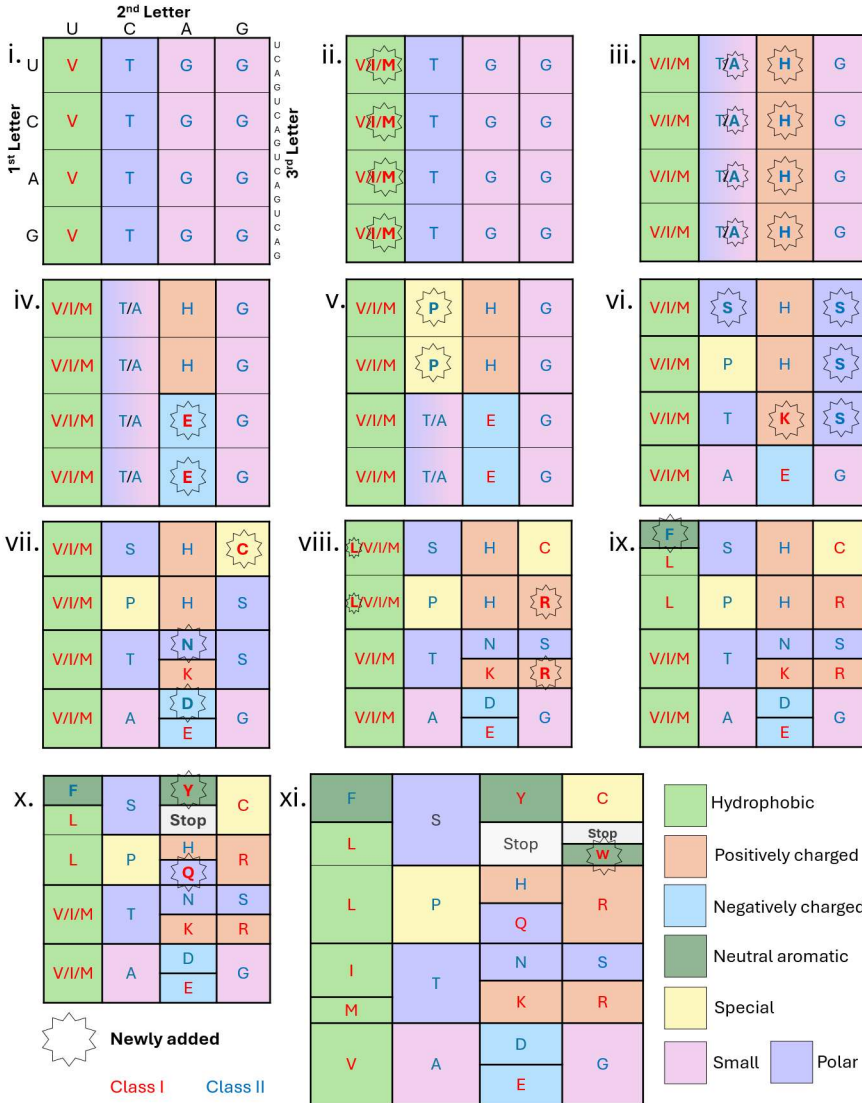
Figure 2. Hypothesized intermediate genetic codes with amino acid ordering from Table 1 LUCA clan usage. Each square indicates four codons spanning all nucleotides in the third position. Past locations of start and stop codons are left as unknown; any codon is expected to act as a stop codon when too little charged tRNA is bound. When we list multiple amino acids for the same codon, it might correspond either to promiscuity, or to unknown status. “Small” amino acids glycine and alanine are deliberately assigned a color close to polar, in recognition of the polar nature of the backbone. “Neutral aromatics” include amino acids with 6-carbon rings (histidine is not always neutral). We assigned these a color close to other hydrophobic amino acids, emphasizing their row rather than column pattern. Other possible categories are amides (i.e. hydrogen bond acceptors) NQ, found in the third column and nucleophiles (i.e. hydrogen bond donors) SCKUT, found in the first and third rows. HYRDE can also serve as nucleophiles in some circumstances.
