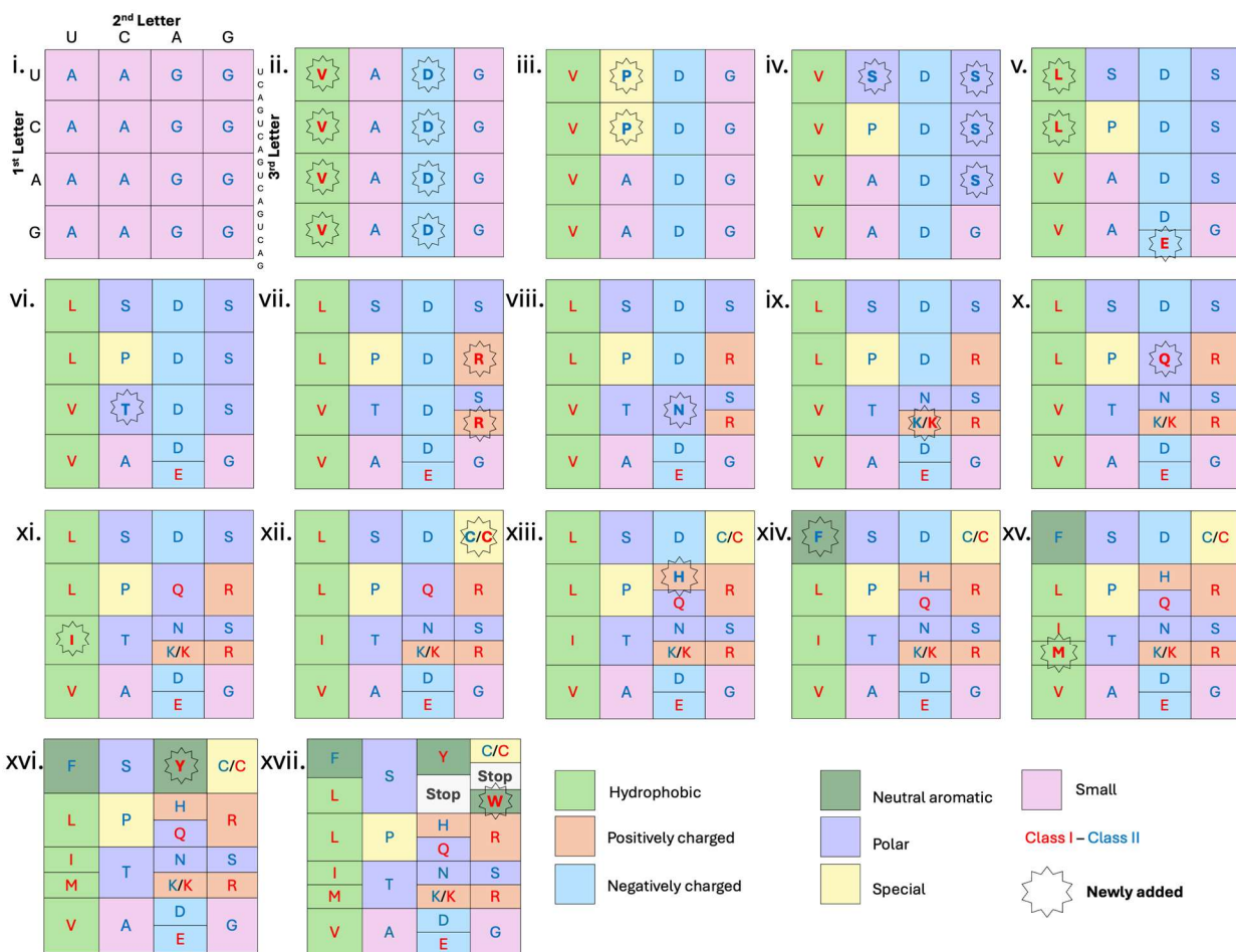
Figure 3. Intermediate genetic codes generated using Trifonov's ordering, as a control analysis. The same scheme is used as in Figure 2.
