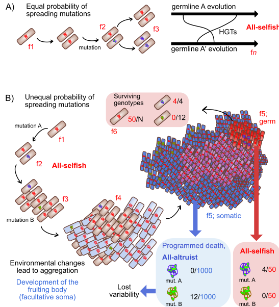
Figure 3. Unitary and partitioned propagation in an extended germline framework.
