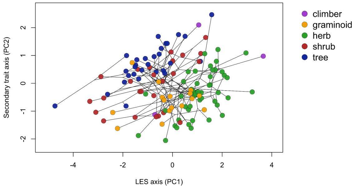
Figure 3. Evolutionary trajectories through multidimensional leaf economics spectrum (LES) space across vascular plants. Phylomorphospace representation of evolutionary relationships within multidimensional leaf economics spectrum (LES) space across vascular plants. Phylogenetic relationships were projected into principal component trait space using a balanced visualization subset of 125 species (25 species per growth form). Colored points represent major plant growth forms (trees, shrubs, herbs, graminoids, and climbers), while connecting branches indicate phylogenetic relationships among taxa. Major growth forms occupied partially overlapping regions of LES space despite significant ecological differentiation, whereas related taxa frequently remained clustered within local regions of ordination space. The coexistence of overlap among growth forms and localized phylogenetic clustering is consistent with strong phylogenetic structure in LES positioning while indicating substantial ecological redistribution across multidimensional trait space.
