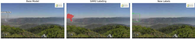
Fig. 3: Labeling workflow: detection by YOLOv11x (left), segmentation propagation with SAM2 (middle), and conversion into refined YOLO bounding boxes (right).
