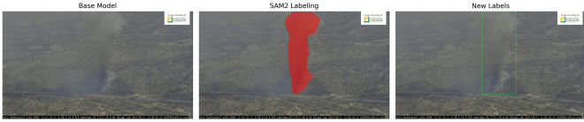
Fig. 4: Example where base YOLOv11x failed to detect smoke, but SAM2, leveraging memory attention, successfully segmented the smoke plume. The segmentation was subsequently converted into YOLO labels.
