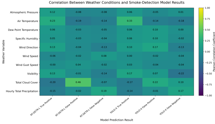
Fig. 18: Pearson correlation coefficients between ignition-hour meteorological variables retrieved through Google Earth Engine [29] and the video-level prediction outcomes of RT-DETR-L[26] and YOLOv11x[21].
