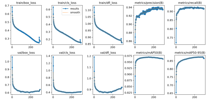
Fig. 11: Training and validation performance for the YOLOv11x model. The first three columns show convergence of Box, Classification, and Distribution Focal loss for both training (top) and validation (bottom) sets. The final two columns display primary accuracy metrics: Precision, Recall, mAP@50, and mAP@50–95. Performance stabilizes after approximately 120 epochs, reaching a precision of 0.94 and mAP@50 of 0.97, indicating robust generalization across diverse wildfire smoke conditions.
