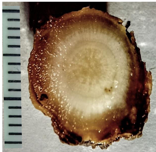
Figure 4H. Taproot cross section showing two 2° xylem growth rings. The central circle with a stellate appearance is the 1° xylem (stele).
