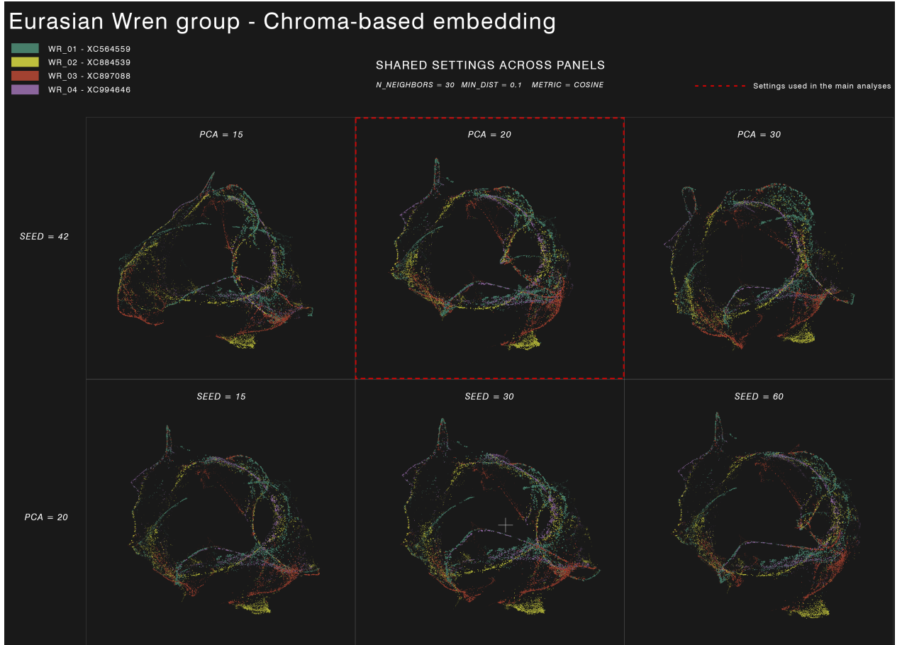
Figure S5: Seed and PCA stability checks for the Eurasian Wren group chroma-based embedding. Top row: PCA dimensionality varied (15, 20, 30) with seed fixed at 42 and canonical UMAP settings ( n\_neighbors = 30 , min\_dist = 0.1 , cosine metric). Bottom row: alternative seed values (15, 30, 60) shown with PCA fixed at 20 and canonical UMAP settings. The red dashed outline marks the canonical setting used in the main analyses ( seed = 42 , PCA = 20 , n\_neighbors = 30 , min\_dist = 0.1 ).
