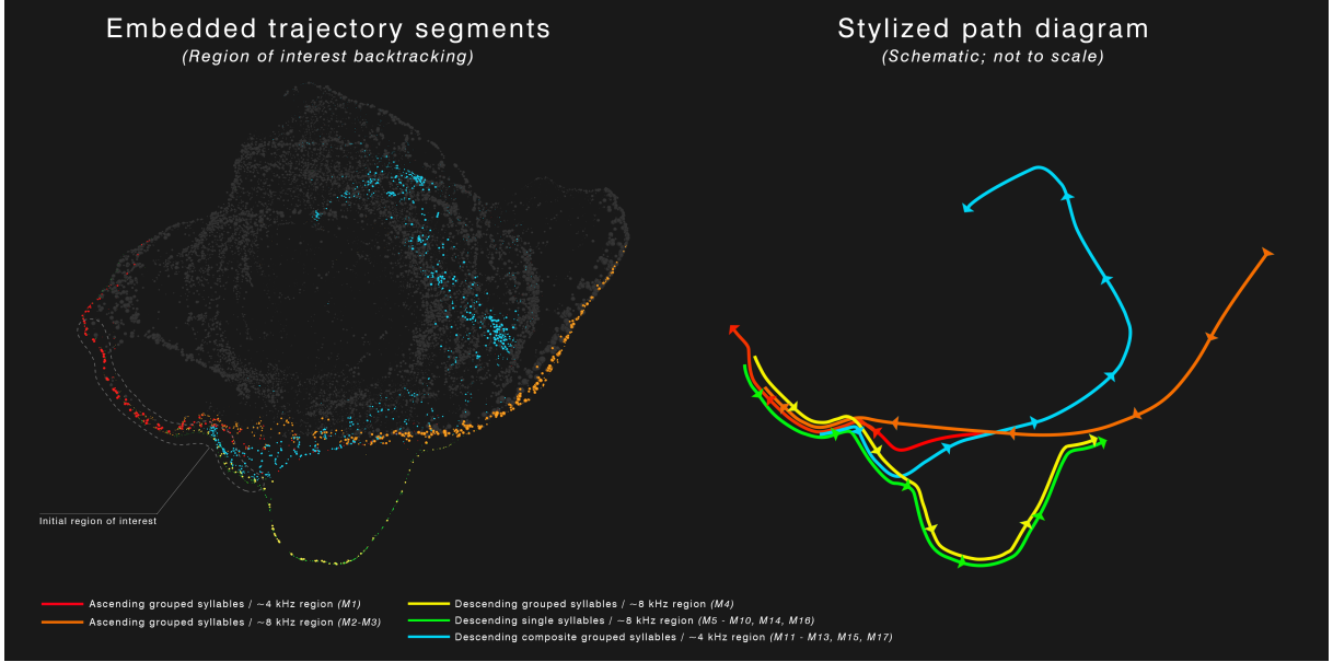
Figure 8: Event-derived trajectory segments and schematic path diagram. Trajectory segments corresponding to the events in Fig. 7 projected back into the full chroma-based manifold. Colored points indicate event-associated frames grouped by contour family and frequency region; the remaining manifold is shown in low opacity for context. The grey dashed outline indicates the initial ROI used for backtracking. Right: stylized path diagram summarizing the dominant shared ridge and branch directions (schematic; not to scale).
