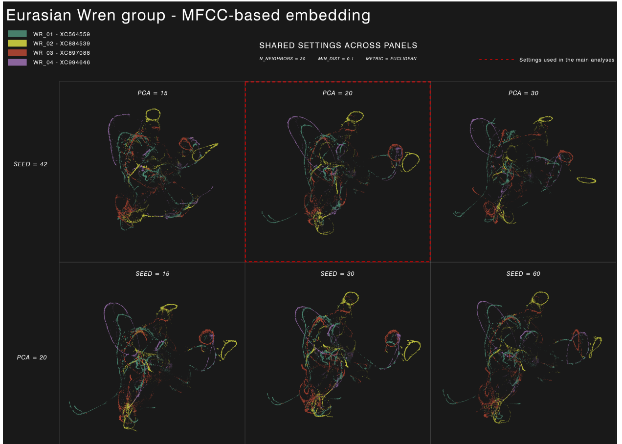
Figure S4: Seed and PCA stability checks for the Eurasian Wren group MFCC-based embedding. Top row: PCA dimensionality varied (15, 20, 30) with seed fixed at 42 and canonical UMAP settings ( n\_neighbors = 30 , min\_dist = 0.1 , Euclidean metric). Bottom row: alternative seed values (15, 30, 60) shown with PCA fixed at 20 and canonical UMAP settings. The red dashed outline marks the canonical setting used in the main analyses ( seed = 42 , PCA = 20 , n\_neighbors = 30 , min\_dist = 0.1 ).
