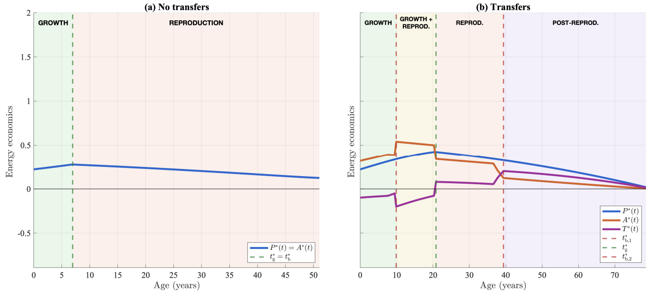
Figure 2: Uninivable life history phases and energy economics under the two budget constraints. Panel (a): without transfers: two phases, juvenile growth (green area) followed by reproduction (red area), with production equal to assimilation throughout ( P^*(t) = A^*(t) , blue line). Panel (b): with transfers without age-specific energy balance ( P^*(t) \neq A^*(t) , blue and red lines), two new phases emerge: continued growth after reproduction (yellow area) and a post-reproductive phase (purple area). Individuals are net-energy consumers until growth stops ( T^*(t) < 0 , negative, purple line). Parameter values and scaling details are given as in Figure 1.
