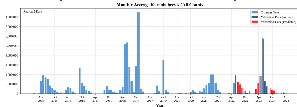
Figure 4: Cross-validation of the validation data for Region 2
