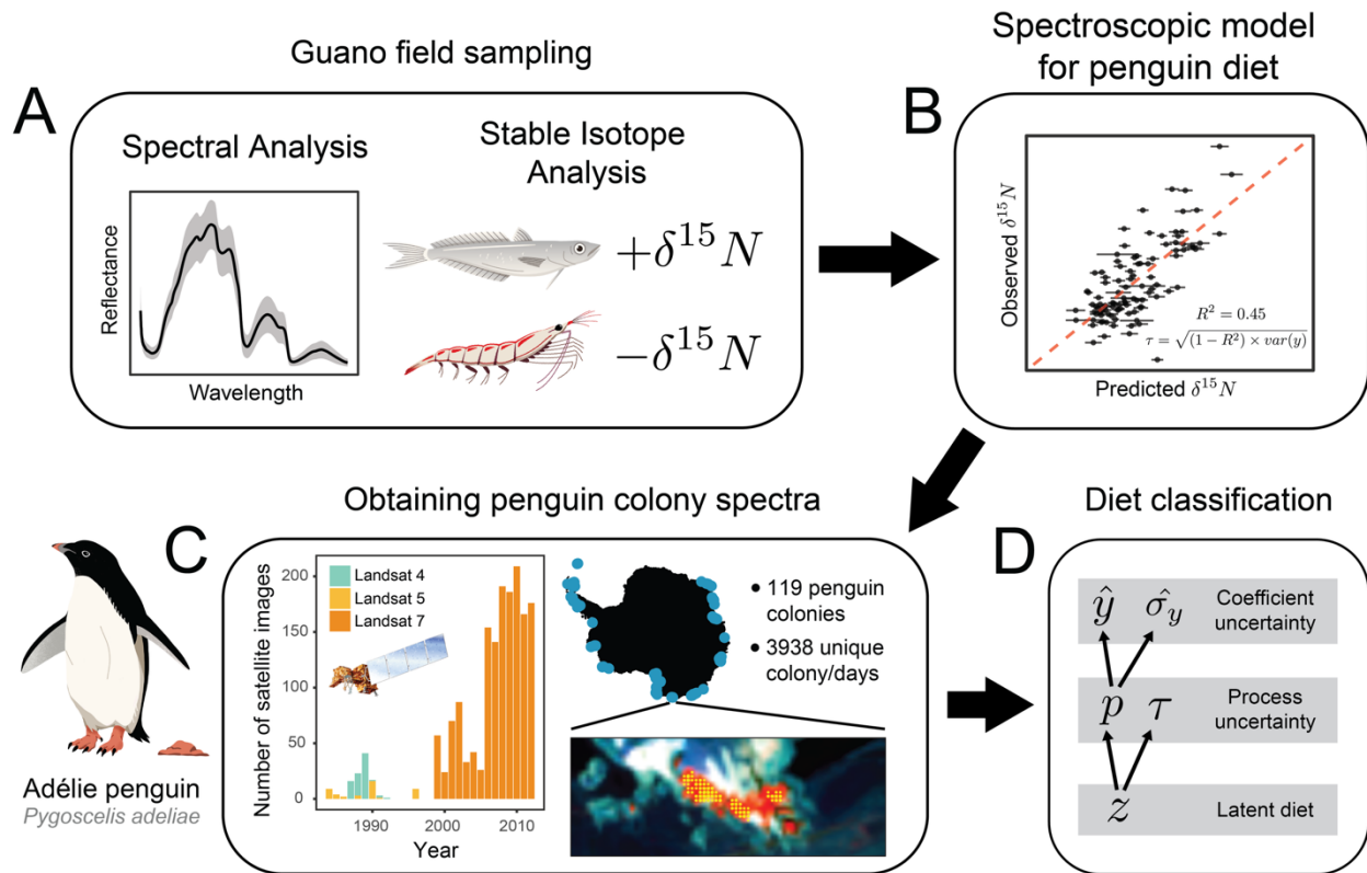
Fig. 1. Integrating approaches from multiple fields, we developed a novel analytical pipeline for quantifying the diet of Adélie penguins ( Pygoscelis adeliae ), the most numerous seabird in Antarctica, from satellites. A) We measured both the spectral reflectance and isotopic signatures of 103 guano samples collected at penguin colonies. Stable nitrogen isotope values ( \delta^{15}N ) indicated the trophic level at which birds were feeding with lower (-) values representing relatively more krill and higher (+) values, more fish. B) We built quantitative models to characterize penguin diet from guano spectra using lab-derived reflectance and stable isotope measurements. C) We applied an algorithmic approach (9) to the Landsat satellite imagery catalog from 1984–2013 to identify and obtain spectral information from guano covered pixels in Adélie penguin colonies across the species global range. D) Using the quantitative model from B we quantify penguin diet for all pixels identified in C. We used a hierarchical Bayesian approach to model how penguin diet varied over space and time, accounting for uncertainty in diet estimates due both to the model’s process uncertainty ( \tau ; B) and uncertainty regarding the coefficients of that model [Eqs. 2–10]. Arrows represent parameter dependencies in the hierarchical model as a Directed Acyclic Graph.
