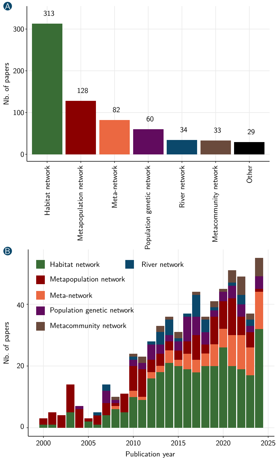
Figure 2: Total (A) and annual (B) number of papers published from 2000 to 2024 using each type of spatial networks considered in this review ( n = 679 ). See Table 1 and Supplementary Information for a description of the spatial networks. The category "Other" includes dispersal networks, spatial networks, and two reviews about networks in ecology.
