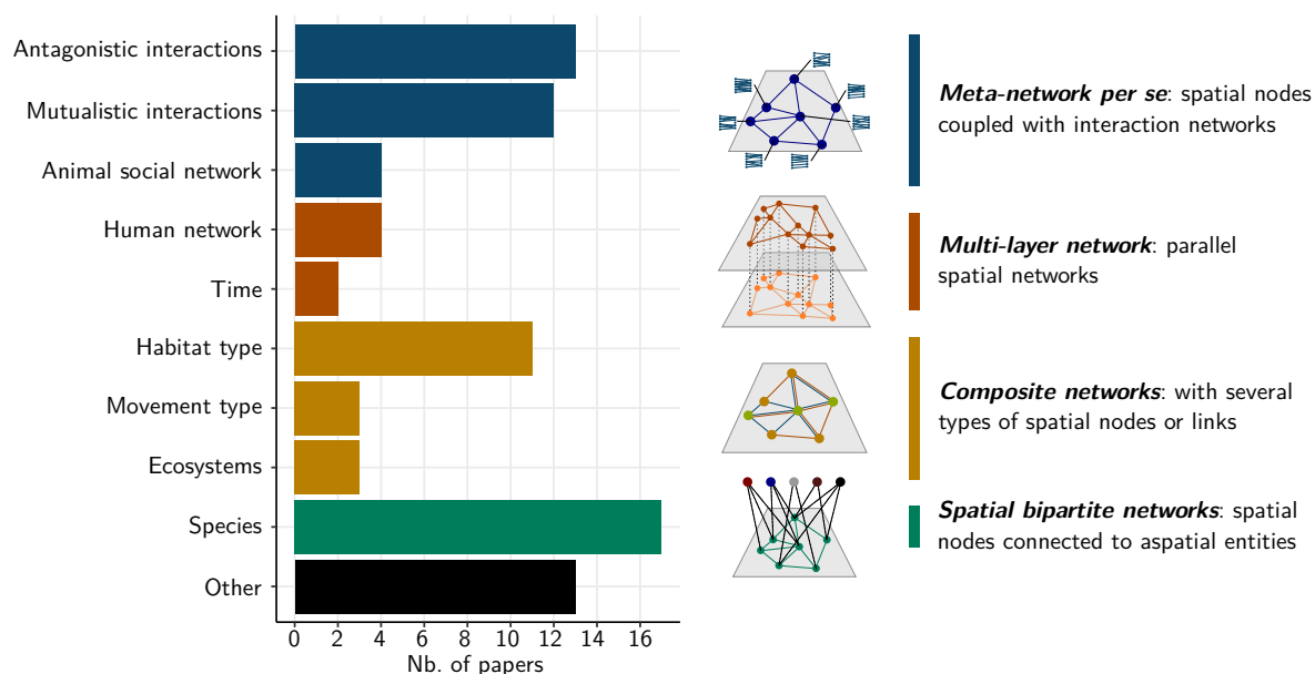
Figure 5: Number of papers about meta-networks of each type. Meta-networks include a spatial network which is either related to node-level interaction networks ( meta-network per se , blue bars), or other spatial layers ( multi-layer network , orange), has several types of nodes or links ( composite network , yellow), or whose nodes are connected to aspatial entities ( spatial bipartite network , green). Interactions include antagonistic interactions (trophic, parasitic), mutualistic interactions (pollination, seed-dispersal), and animal social networks. Multi-layer networks include temporal layers or human infrastructure networks. Node types can represent habitat types or ecosystems, and link types distinguish movement types. In the considered corpus, aspatial entities related to nodes were species. The "Other" category includes review papers and meta-networks not falling in previous categories.
