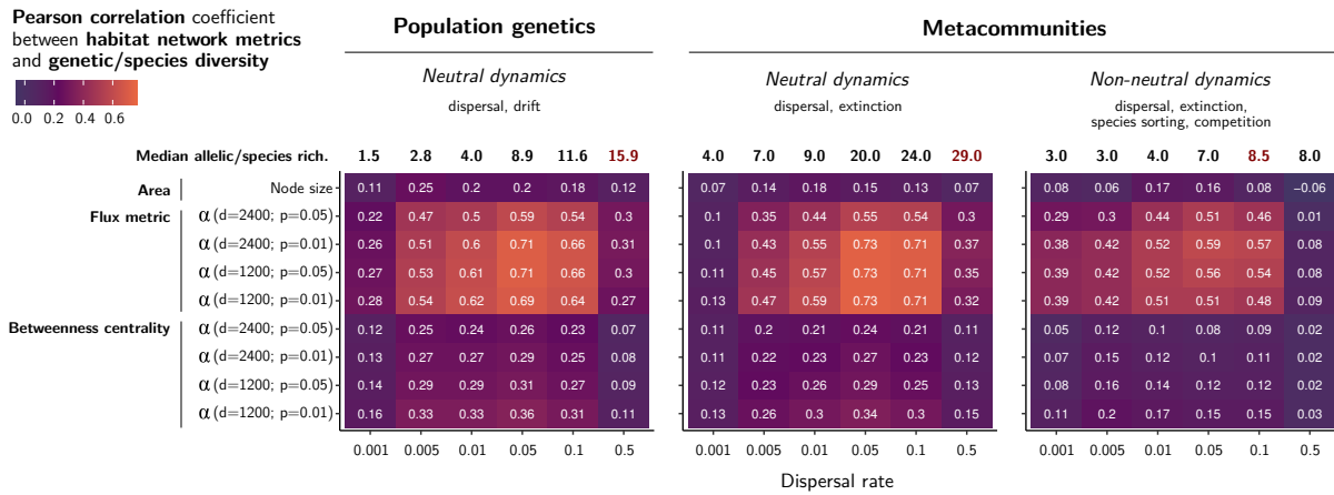
Figure 6: Pearson correlation coefficients between the Area (node size), Flux metric, or Betweenness centrality metric computed at the node-level for each forest patch displayed on Figure 1 (in log-scale) and either the allelic richness of populations (left panels) or species richness of communities (middle and right panels). These responses were simulated in these patches under the action of different ecological or evolutionary processes. Neutral population genetic simulations (left panel) included the effect of genetic drift and dispersal-driven gene flow. Neutral metacommunity simulations (middle panel) included the effect of dispersal, stochastic extinction (i.e., ecological drift), and equal intra- and inter-specific competition. The non-neutral metacommunity simulations (right panel) included species with different niches subject to species sorting, stronger intra- than inter-specific competition (stabilizing), as well as dispersal and stochastic extinction. The x -axis of each heatmap panel distinguishes simulations performed with dispersal rates and probabilities ranging from 0.001 to 0.5 (6 discrete values). The y -axis of each heatmap distinguishes metrics computed at the node level (Area, Flux, Betweenness Centrality), using different parameters for the Flux and Betweenness Centrality metrics. The parameter \alpha used for their computation was set so that the assumed dispersal probability is equal to 0.01 or 0.05 at distances equal to 1,200 or 2,400 cost-distance units. Color variations match variations in Pearson correlation coefficients assessing the strength and direction of the linear relationship between the metrics and the diversity response for n = 610 patches. On top of each panel, the median values of allelic or species richness are indicated for each dispersal rate. See more details in the Supplementary Information and Figure S6 for scatterplots of simulations results..
