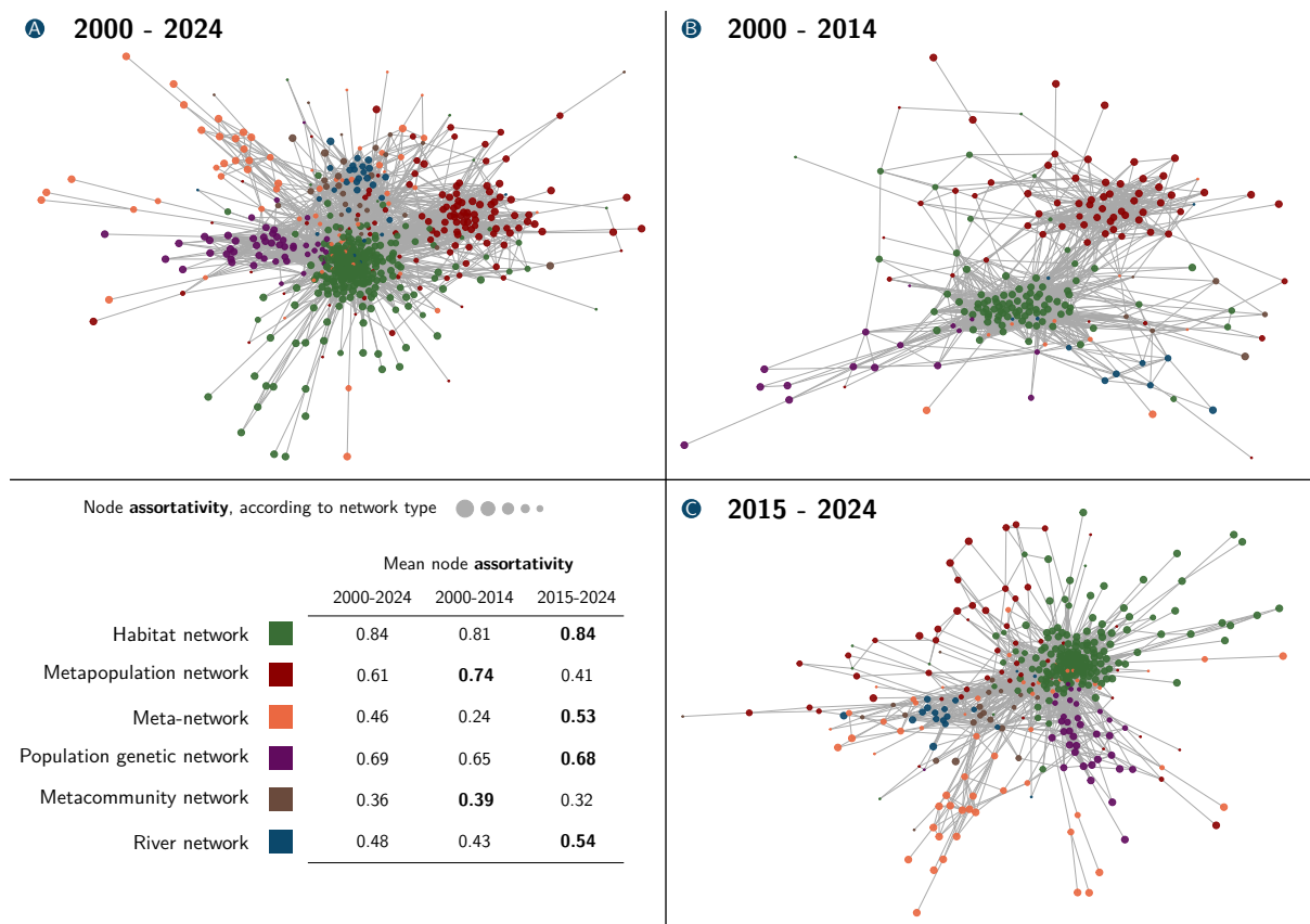
Figure 4: Networks of bibliographic coupling among papers about spatial networks in the whole corpus (A) or published in the periods 2000-2014 (B) or 2015-2024 (C). Each node represents a paper and its color represents the type of spatial network considered in the paper. The links connect papers sharing more than 3 % of their cited references and are weighted by the Jaccard index quantifying the dissimilarity of their citations ( < 0.97 ). Node positions were computed using Jaccard index values computed at link-level to implement the Fruchterman and Reingold algorithm, such that papers sharing similar references are closeby. Node size reflects their assortativity, i.e., the proportion of the connected papers that are about the same type of spatial network as the focal one. The bottom-left table reports the mean assortativity of papers about each spatial network over time.
